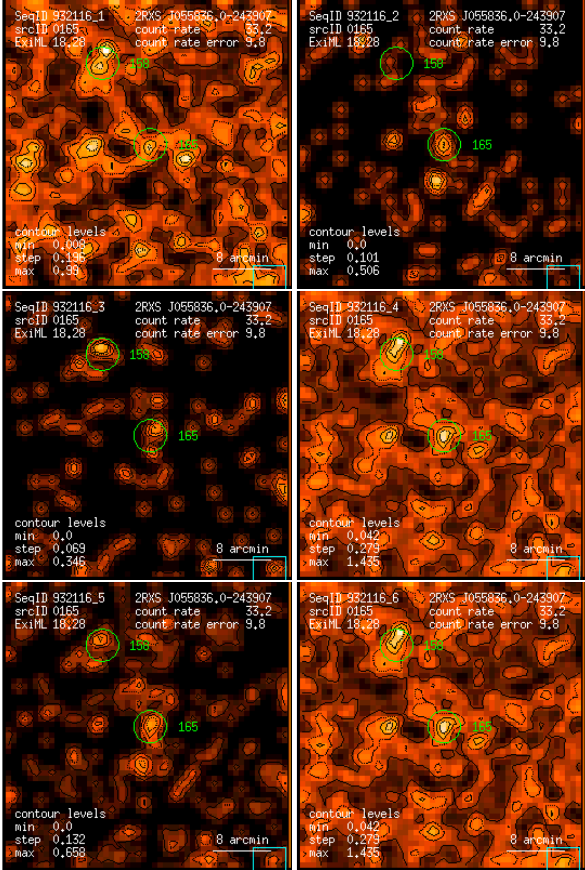
Figure 165: RASS 932116: detection 0165: band rate images, Gaussian filter: (1) PSPC channels 11 – 41, (2) 52 – 90, (3) 91 – 201, (4) 11 – 235, (5) 52 – 201, (6) 11 – 201. Broad band rates in counts/ks. Band rate contour levels in counts/ks/arcmin 2 .
