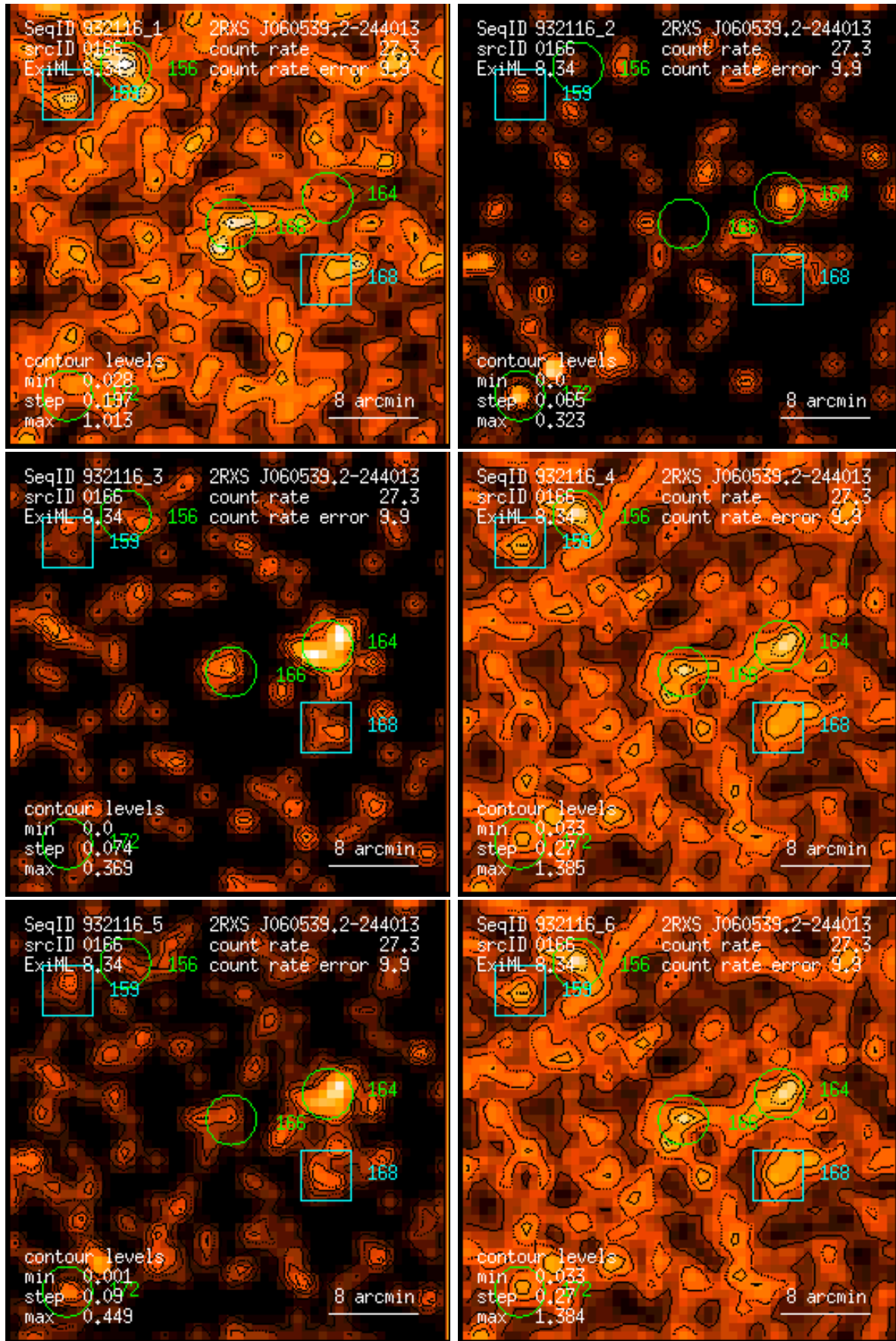
Figure 166: RASS 932116: detection 0166: band rate images, Gaussian filter: (1) PSPC channels 11 – 41, (2) 52 – 90, (3) 91 – 201, (4) 11 – 235, (5) 52 – 201, (6) 11 – 201. Broad band rates in counts/ks. Band rate contour levels in counts/ks/arcmin 2 .
