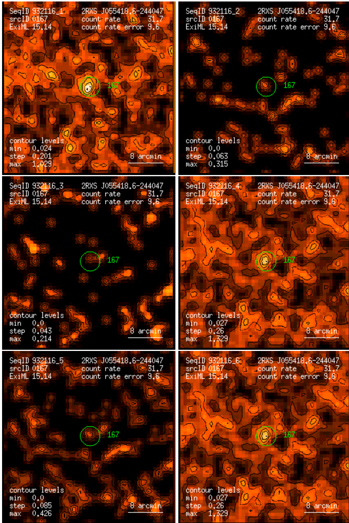
Figure 167: RASS 932116: detection 0167: band rate images, Gaussian filter: (1) PSPC channels 11 – 41, (2) 52 – 90, (3) 91 – 201, (4) 11 – 235, (5) 52 – 201, (6) 11 – 201. Broad band rates in counts/ks. Band rate contour levels in counts/ks/arcmin 2 .
