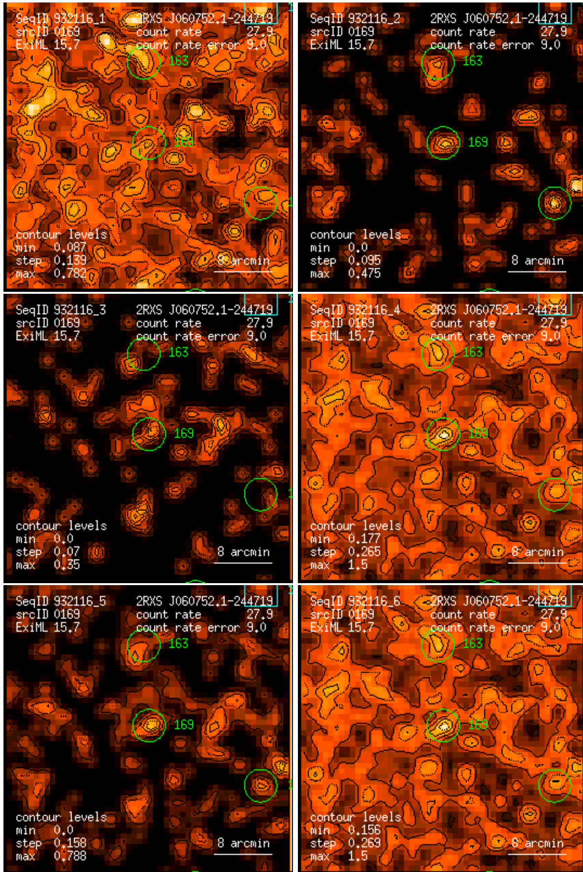
Figure 169: RASS 932116: detection 0169: band rate images, Gaussian filter: (1) PSPC channels 11 – 41, (2) 52 – 90, (3) 91 – 201, (4) 11 – 235, (5) 52 – 201, (6) 11 – 201. Broad band rates in counts/ks. Band rate contour levels in counts/ks/arcmin 2 .
