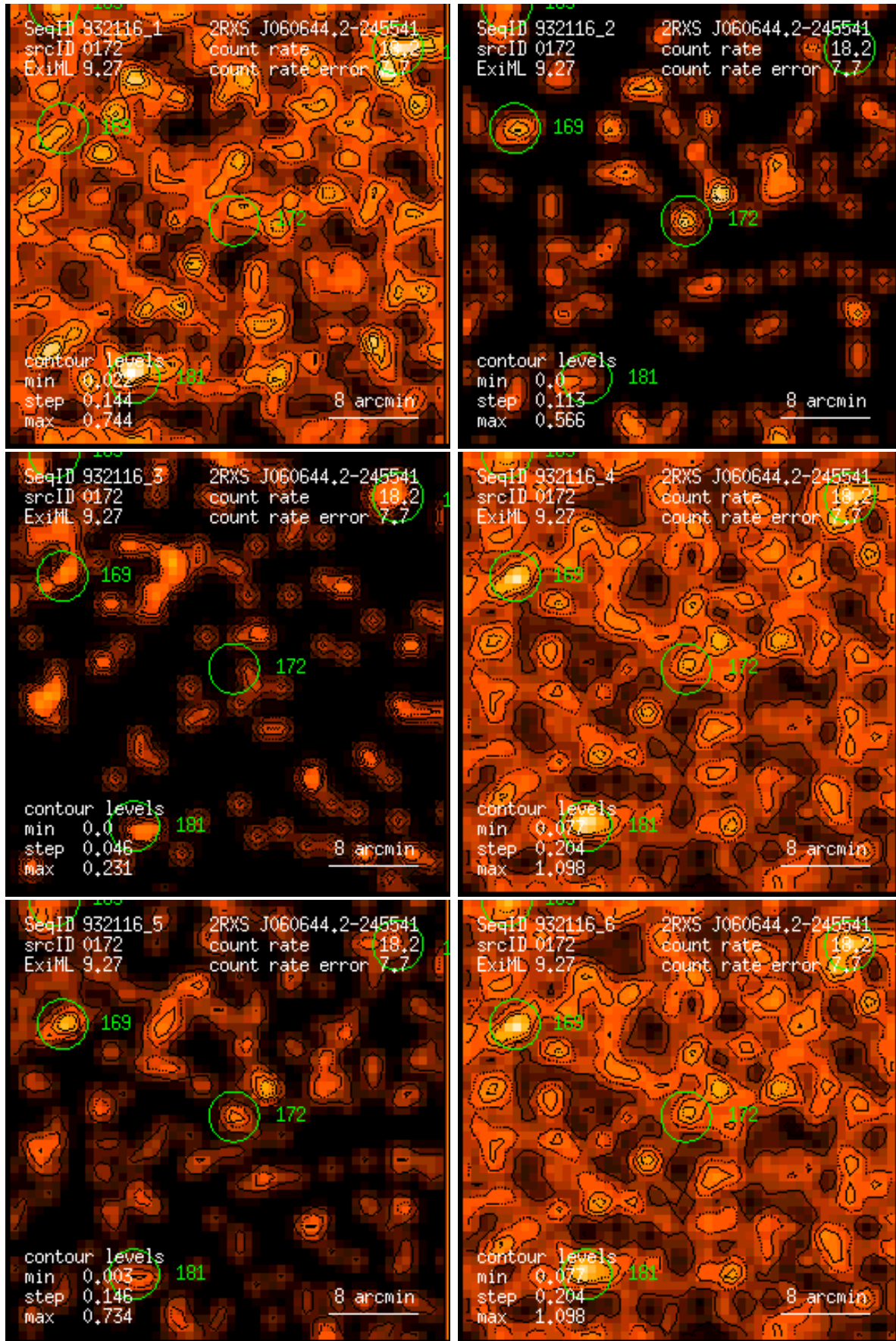
Figure 172: RASS 932116: detection 0172: band rate images, Gaussian filter: (1) PSPC channels 11 – 41, (2) 52 – 90, (3) 91 – 201, (4) 11 – 235, (5) 52 – 201, (6) 11 – 201. Broad band rates in counts/ks. Band rate contour levels in counts/ks/arcmin 2 .
