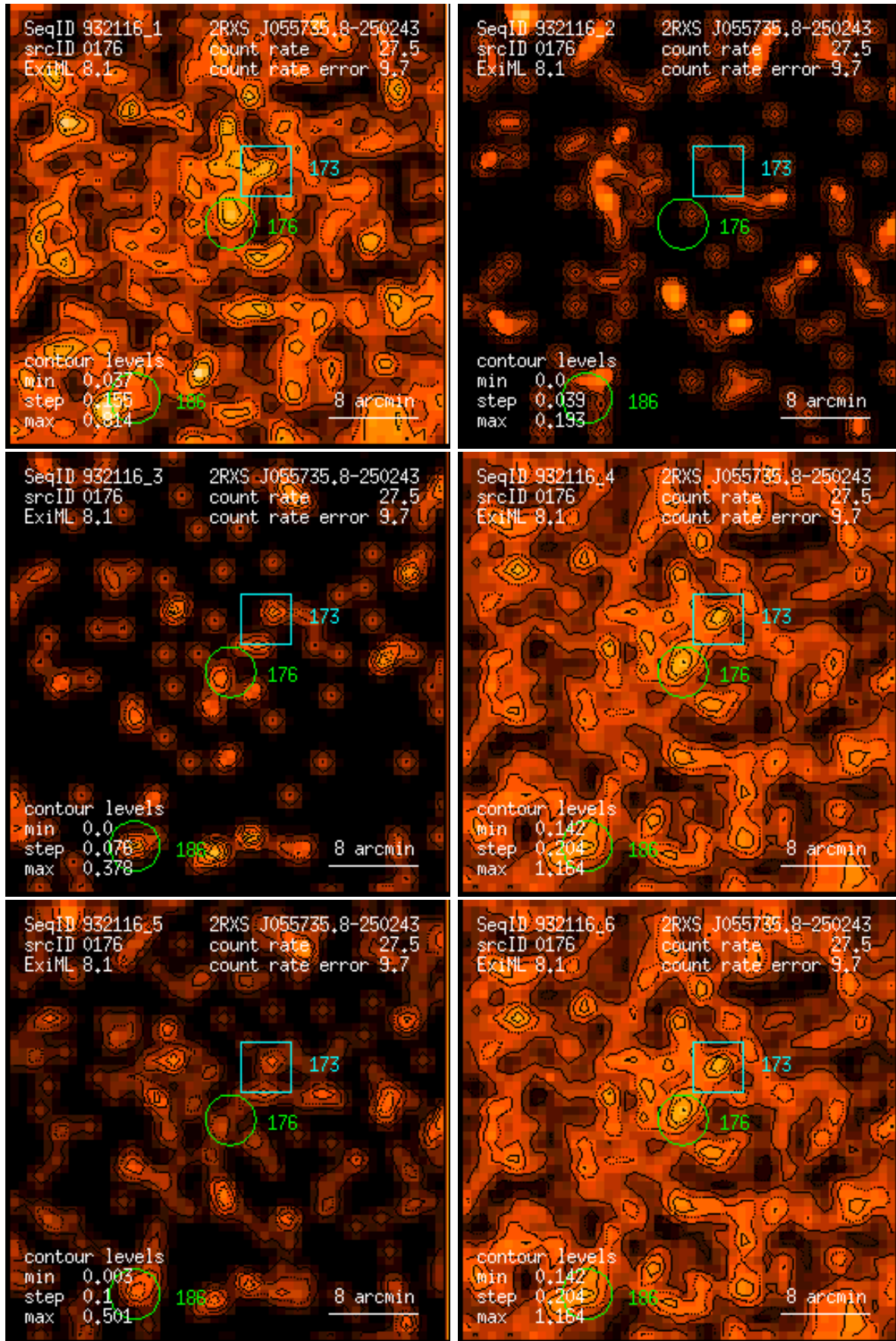
Figure 176: RASS 932116: detection 0176: band rate images, Gaussian filter: (1) PSPC channels 11 – 41, (2) 52 – 90, (3) 91 – 201, (4) 11 – 235, (5) 52 – 201, (6) 11 – 201. Broad band rates in counts/ks. Band rate contour levels in counts/ks/arcmin 2 .
