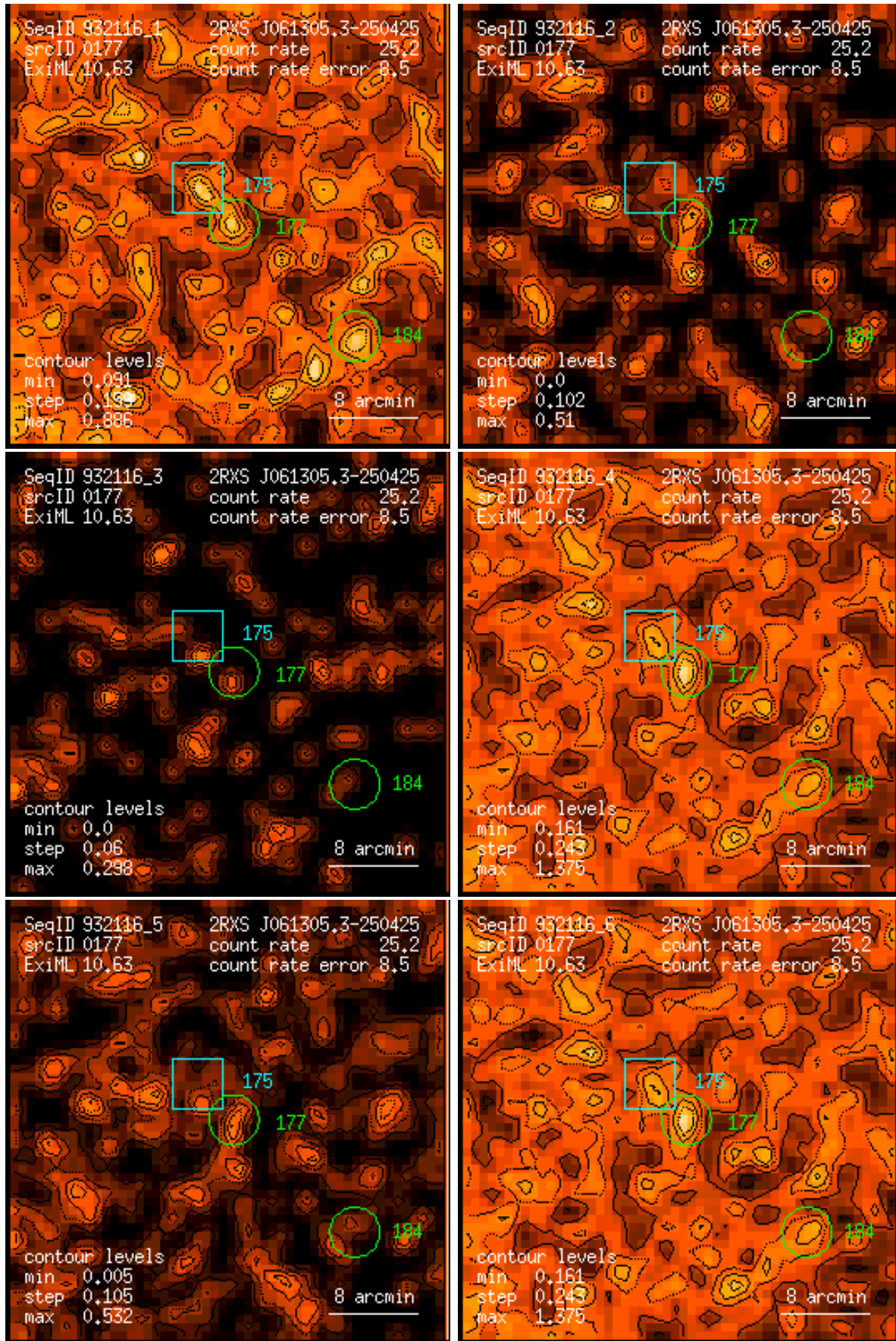
Figure 177: RASS 932116: detection 0177: band rate images, Gaussian filter: (1) PSPC channels 11 – 41, (2) 52 – 90, (3) 91 – 201, (4) 11 – 235, (5) 52 – 201, (6) 11 – 201. Broad band rates in counts/ks. Band rate contour levels in counts/ks/arcmin 2 .
