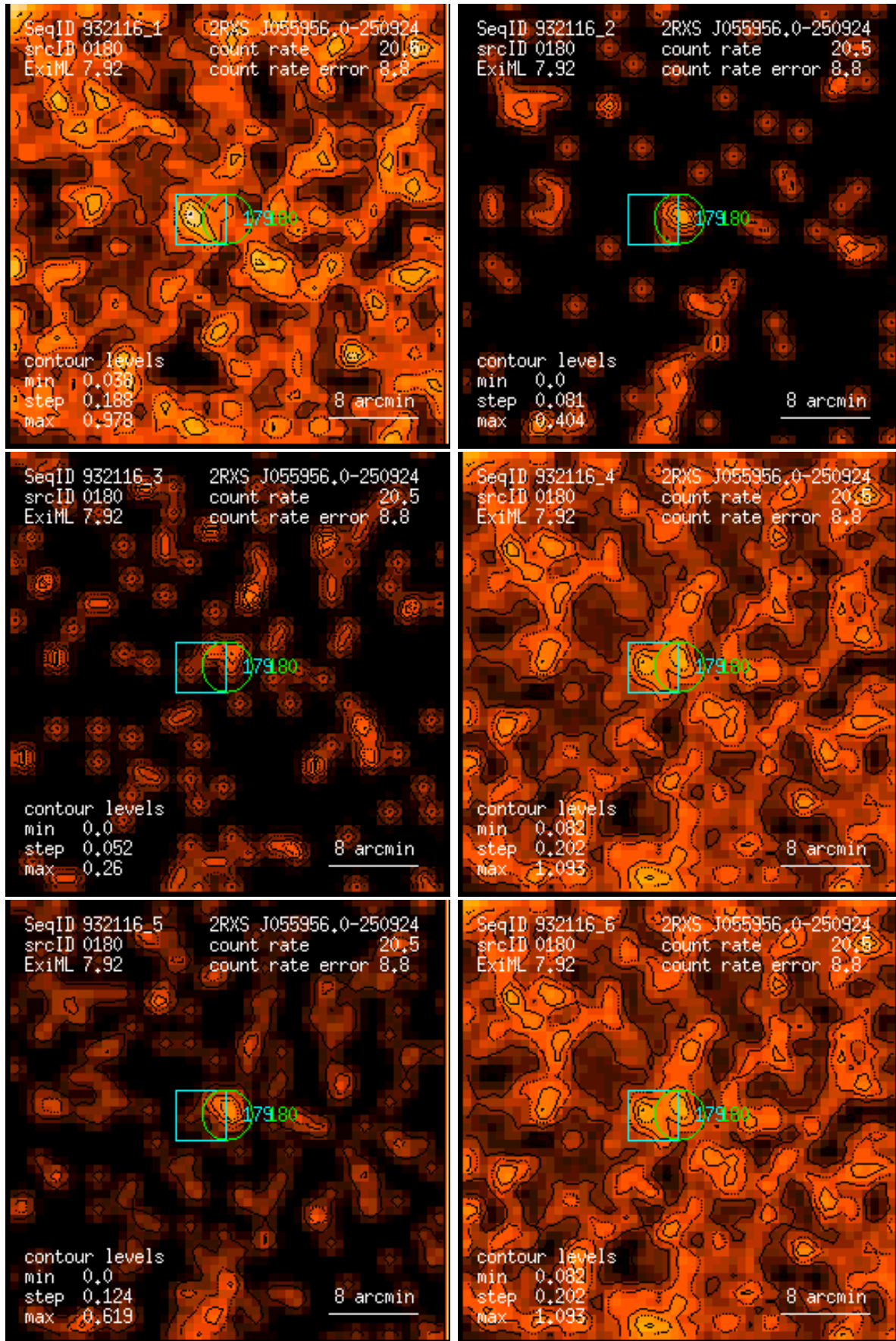
Figure 180: RASS 932116: detection 0180: band rate images, Gaussian filter: (1) PSPC channels 11 – 41, (2) 52 – 90, (3) 91 – 201, (4) 11 – 235, (5) 52 – 201, (6) 11 – 201. Broad band rates in counts/ks. Band rate contour levels in counts/ks/arcmin 2 .
