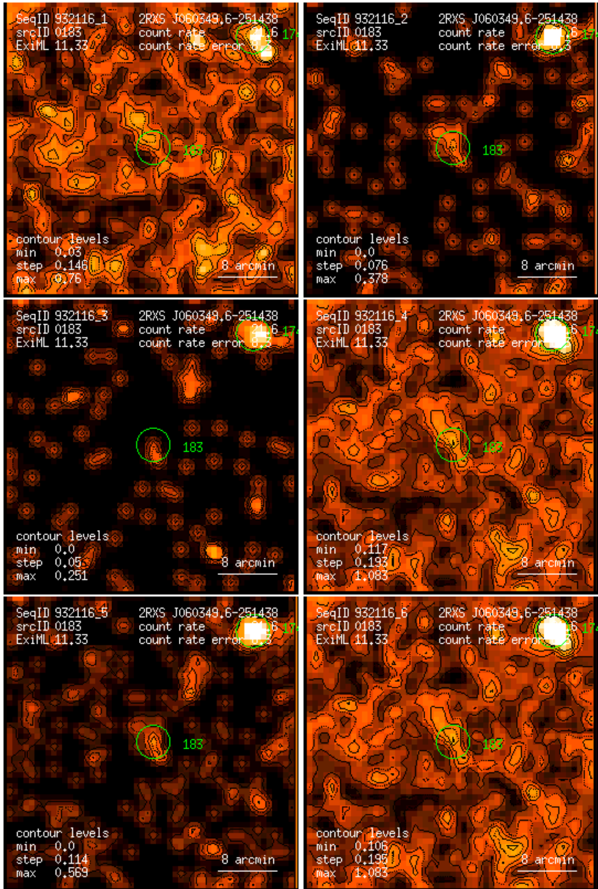
Figure 183: RASS 932116: detection 0183: band rate images, Gaussian filter: (1) PSPC channels 11 – 41, (2) 52 – 90, (3) 91 – 201, (4) 11 – 235, (5) 52 – 201, (6) 11 – 201. Broad band rates in counts/ks. Band rate contour levels in counts/ks/arcmin 2 .
