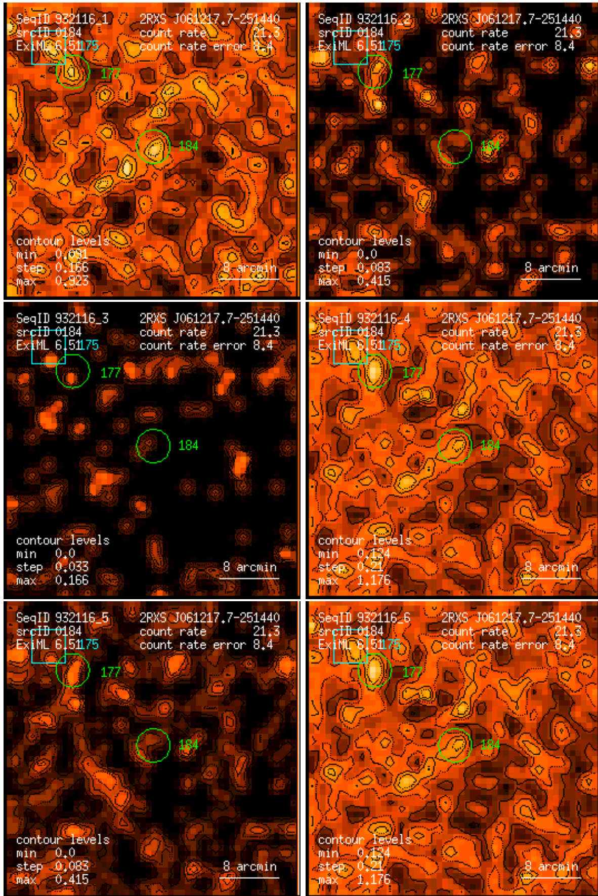
Figure 184: RASS 932116: detection 0184: band rate images, Gaussian filter: (1) PSPC channels 11 – 41, (2) 52 – 90, (3) 91 – 201, (4) 11 – 235, (5) 52 – 201, (6) 11 – 201. Broad band rates in counts/ks. Band rate contour levels in counts/ks/arcmin 2 .
