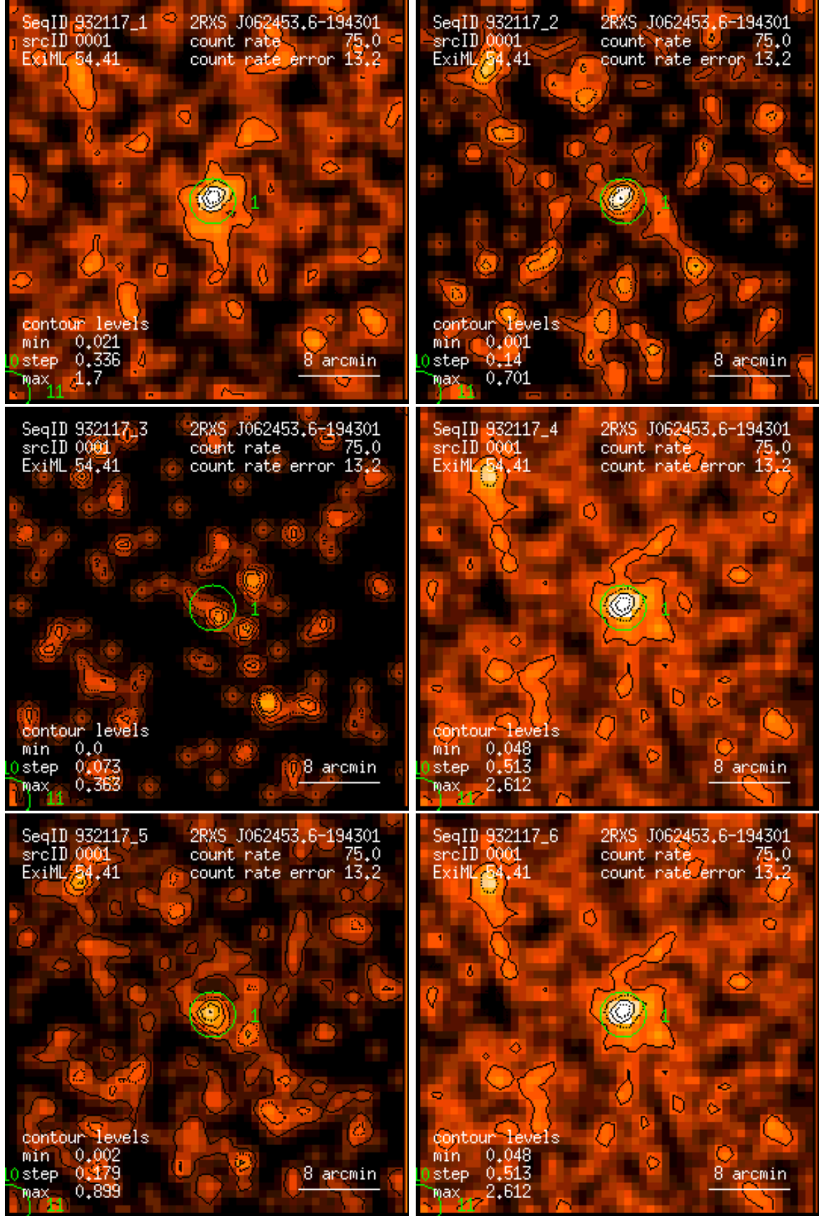
Figure 1: RASS 932117: detection 0001: band rate images, Gaussian filter: (1) PSPC channels 11 – 41, (2) 52 – 90, (3) 91 – 201, (4) 11 – 235, (5) 52 – 201, (6) 11 – 201. Broad band rates in counts/ks. Band rate contour levels in counts/ks/arcmin 2 .
