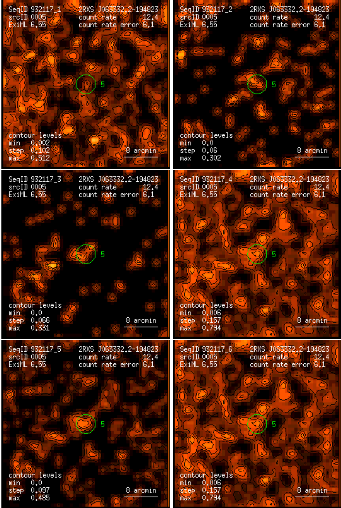
Figure 5: RASS 932117: detection 0005: band rate images, Gaussian filter: (1) PSPC channels 11 – 41, (2) 52 – 90, (3) 91 – 201, (4) 11 – 235, (5) 52 – 201, (6) 11 – 201. Broad band rates in counts/ks. Band rate contour levels in counts/ks/arcmin 2 .
