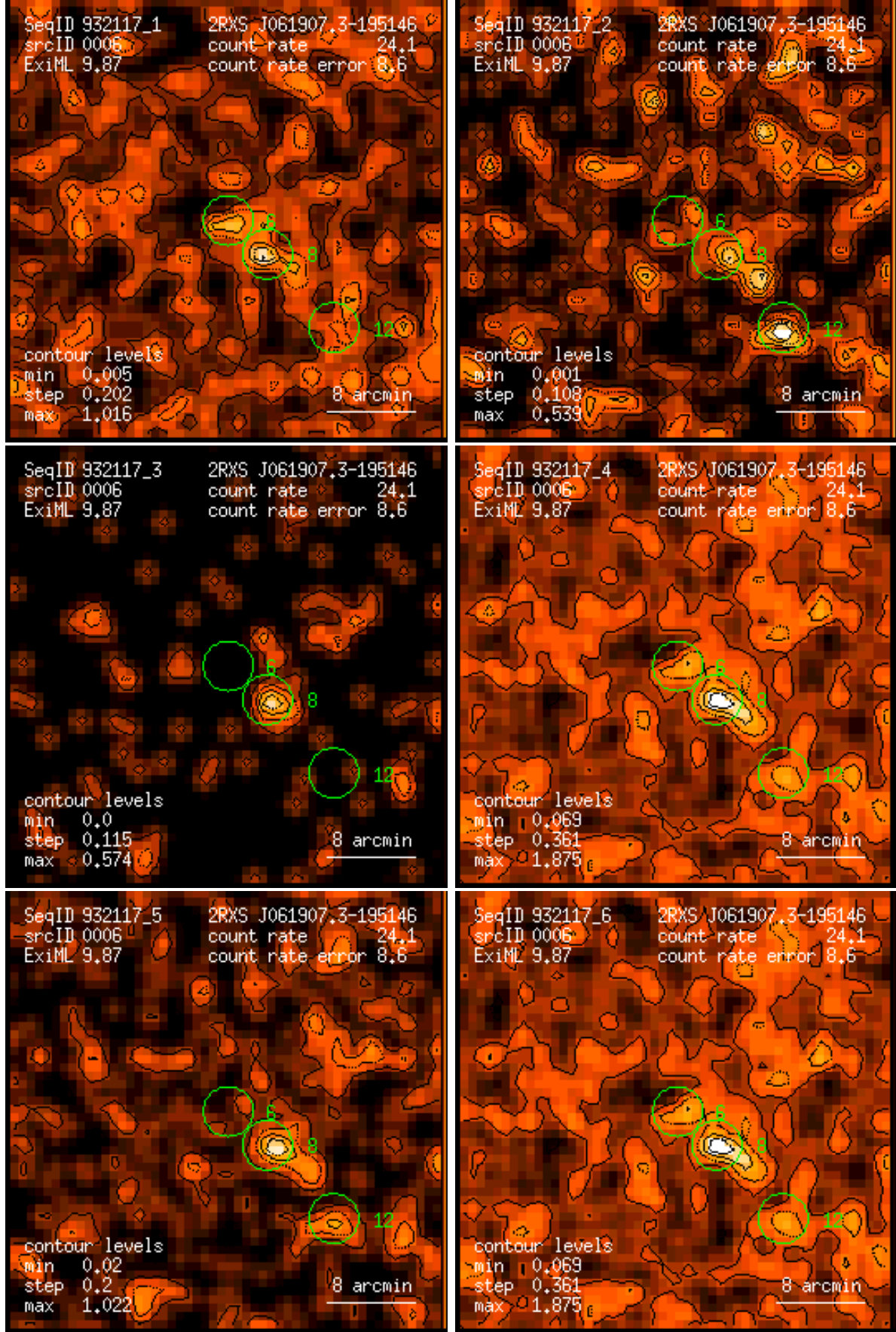
Figure 6: RASS 932117: detection 0006: band rate images, Gaussian filter: (1) PSPC channels 11 – 41, (2) 52 – 90, (3) 91 – 201, (4) 11 – 235, (5) 52 – 201, (6) 11 – 201. Broad band rates in counts/ks. Band rate contour levels in counts/ks/arcmin 2 .
