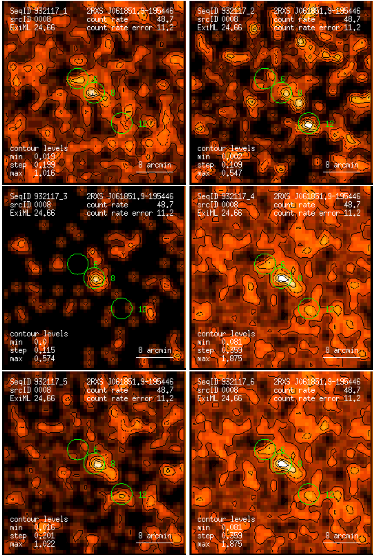
Figure 8: RASS 932117: detection 0008: band rate images, Gaussian filter: (1) PSPC channels 11 – 41, (2) 52 – 90, (3) 91 – 201, (4) 11 – 235, (5) 52 – 201, (6) 11 – 201. Broad band rates in counts/ks. Band rate contour levels in counts/ks/arcmin 2 .
