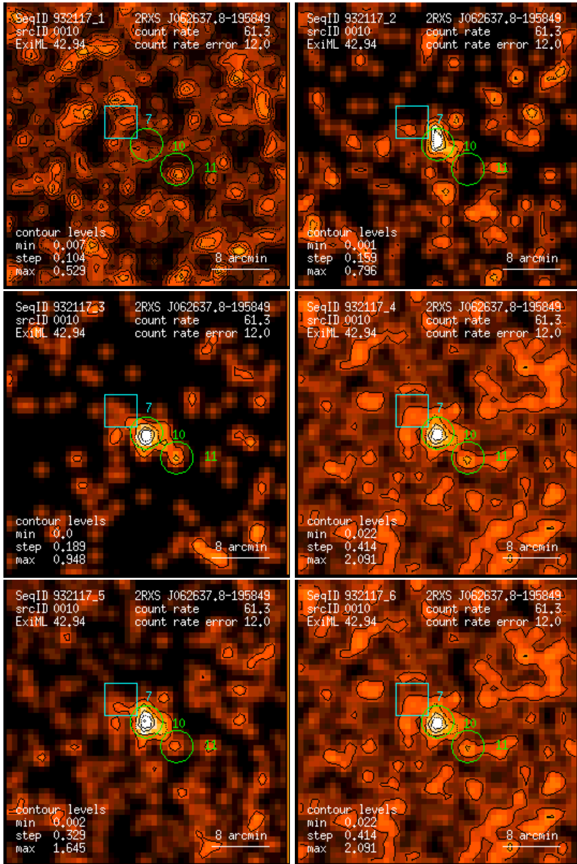
Figure 10: RASS 932117: detection 0010: band rate images, Gaussian filter: (1) PSPC channels 11 – 41, (2) 52 – 90, (3) 91 – 201, (4) 11 – 235, (5) 52 – 201, (6) 11 – 201. Broad band rates in counts/ks. Band rate contour levels in counts/ks/arcmin 2 .
