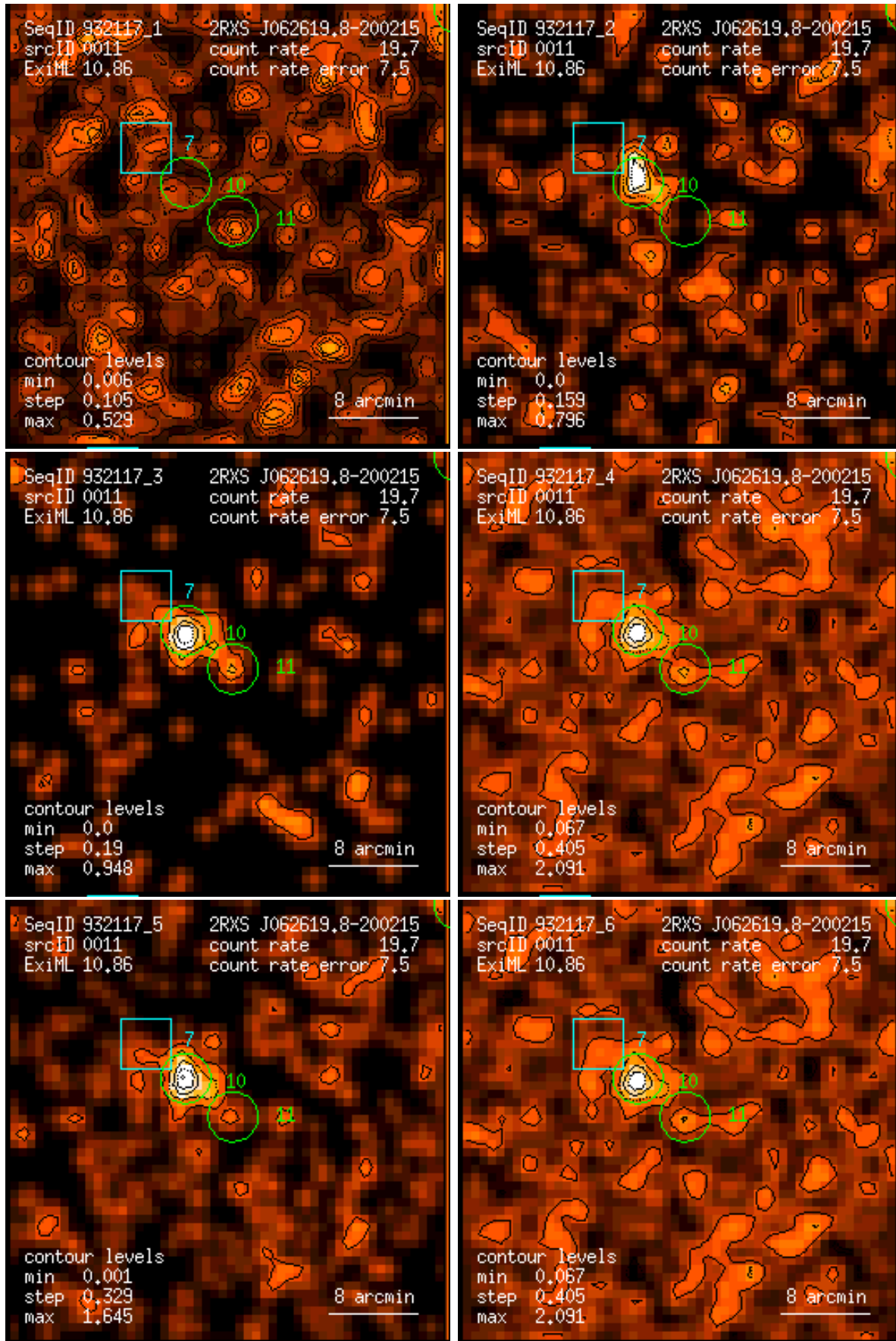
Figure 11: RASS 932117: detection 0011: band rate images, Gaussian filter: (1) PSPC channels 11 – 41, (2) 52 – 90, (3) 91 – 201, (4) 11 – 235, (5) 52 – 201, (6) 11 – 201. Broad band rates in counts/ks. Band rate contour levels in counts/ks/arcmin 2 .
