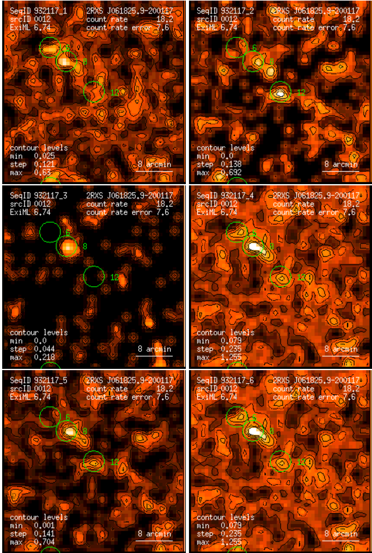
Figure 12: RASS 932117: detection 0012: band rate images, Gaussian filter: (1) PSPC channels 11 – 41, (2) 52 – 90, (3) 91 – 201, (4) 11 – 235, (5) 52 – 201, (6) 11 – 201. Broad band rates in counts/ks. Band rate contour levels in counts/ks/arcmin 2 .
