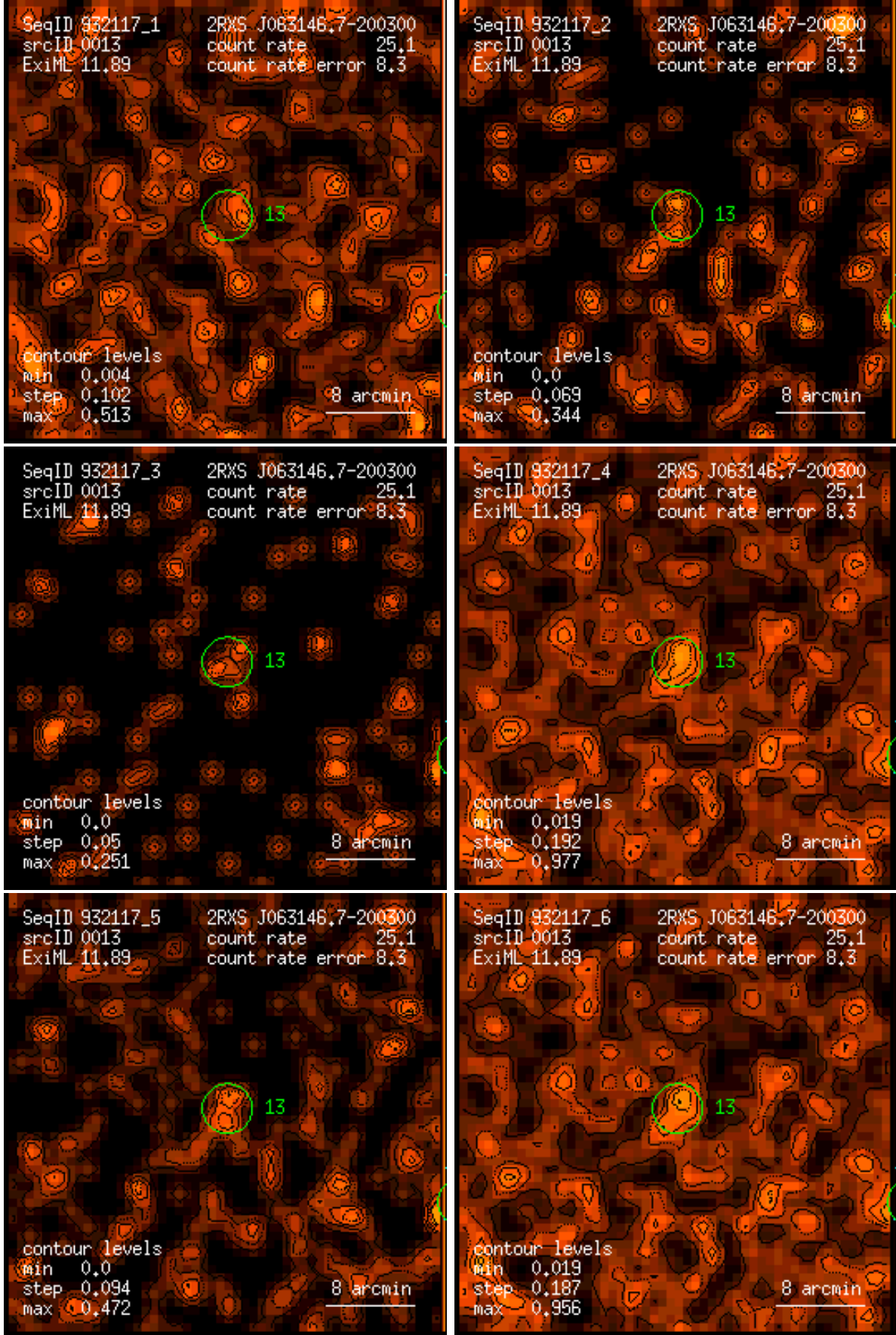
Figure 13: RASS 932117: detection 0013: band rate images, Gaussian filter: (1) PSPC channels 11 – 41, (2) 52 – 90, (3) 91 – 201, (4) 11 – 235, (5) 52 – 201, (6) 11 – 201. Broad band rates in counts/ks. Band rate contour levels in counts/ks/arcmin 2 .
