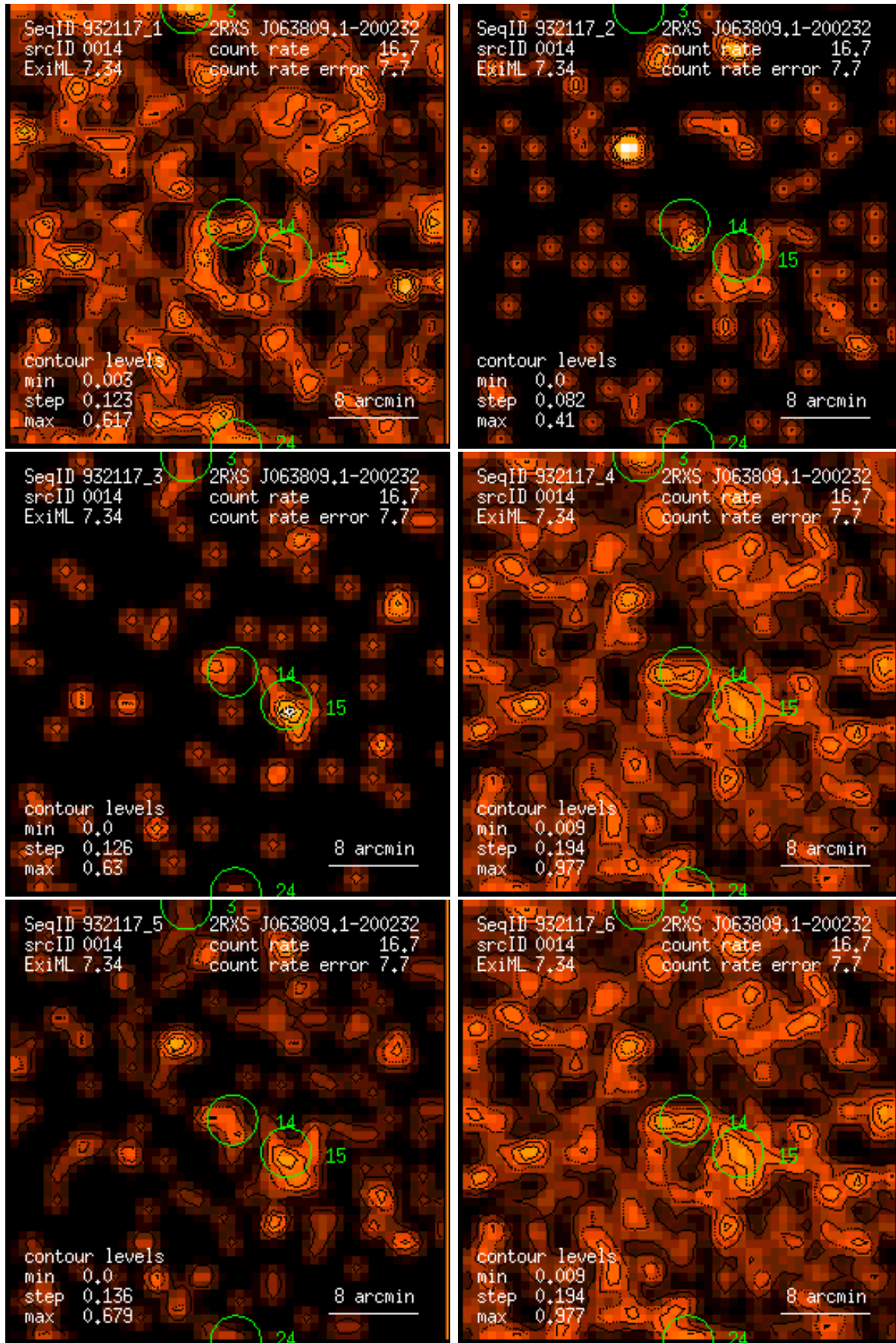
Figure 14: RASS 932117: detection 0014: band rate images, Gaussian filter: (1) PSPC channels 11 – 41, (2) 52 – 90, (3) 91 – 201, (4) 11 – 235, (5) 52 – 201, (6) 11 – 201. Broad band rates in counts/ks. Band rate contour levels in counts/ks/arcmin 2 .
