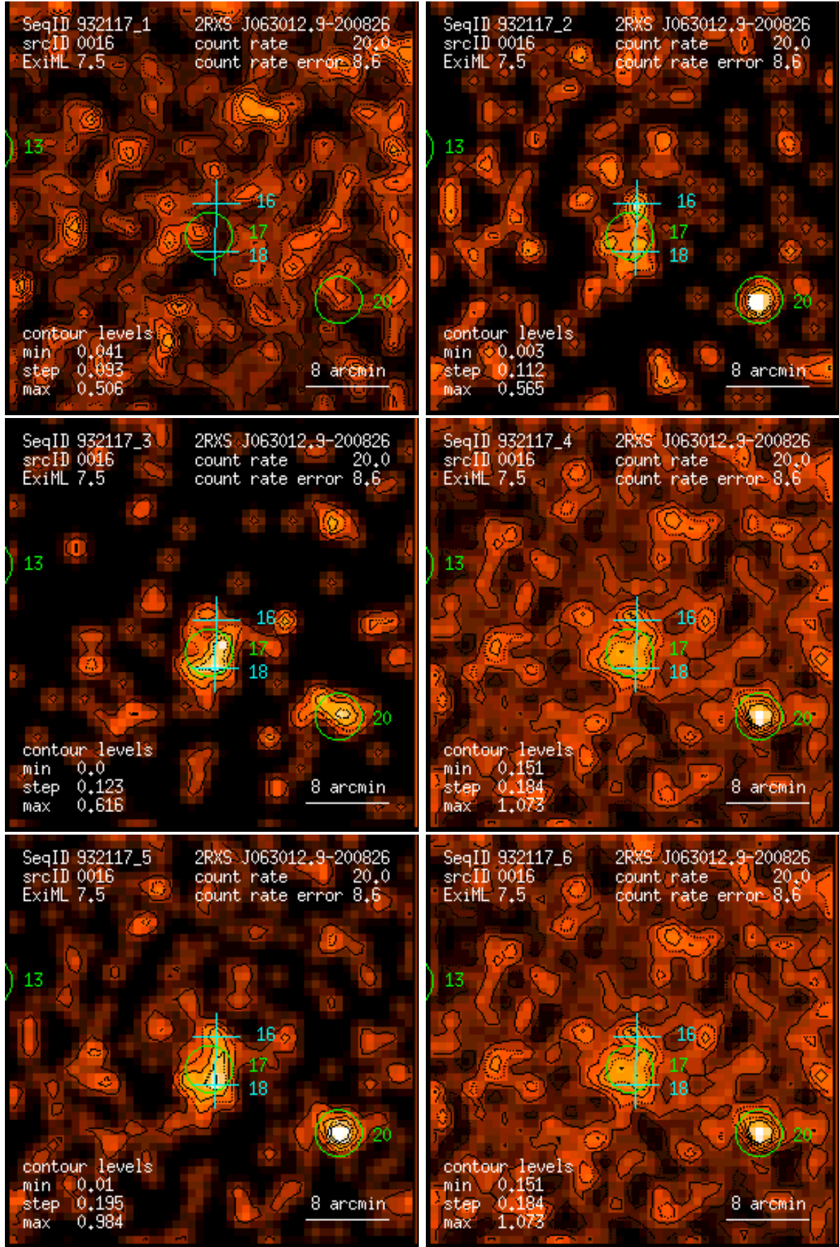
Figure 16: RASS 932117: detection 0016: band rate images, Gaussian filter: (1) PSPC channels 11 – 41, (2) 52 – 90, (3) 91 – 201, (4) 11 – 235, (5) 52 – 201, (6) 11 – 201. Broad band rates in counts/ks. Band rate contour levels in counts/ks/arcmin 2 .
