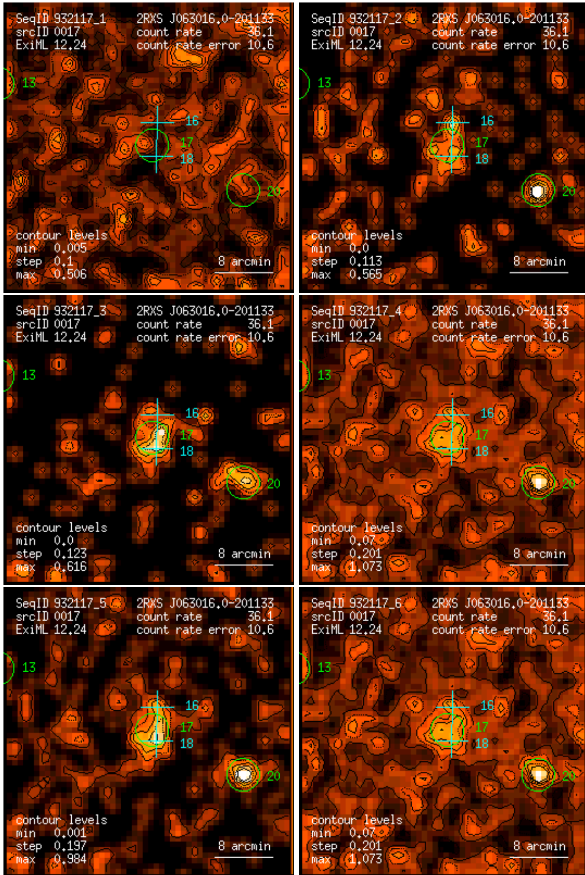
Figure 17: RASS 932117: detection 0017: band rate images, Gaussian filter: (1) PSPC channels 11 – 41, (2) 52 – 90, (3) 91 – 201, (4) 11 – 235, (5) 52 – 201, (6) 11 – 201. Broad band rates in counts/ks. Band rate contour levels in counts/ks/arcmin 2 .
