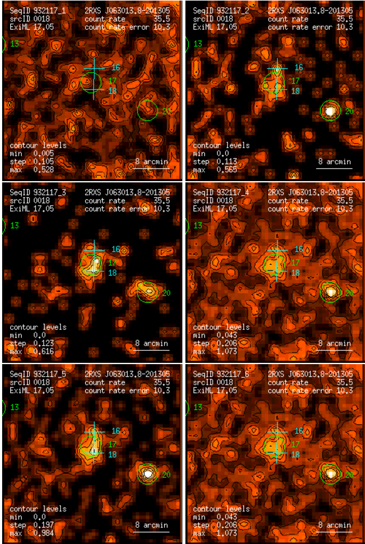
Figure 18: RASS 932117: detection 0018: band rate images, Gaussian filter: (1) PSPC channels 11 – 41, (2) 52 – 90, (3) 91 – 201, (4) 11 – 235, (5) 52 – 201, (6) 11 – 201. Broad band rates in counts/ks. Band rate contour levels in counts/ks/arcmin 2 .
