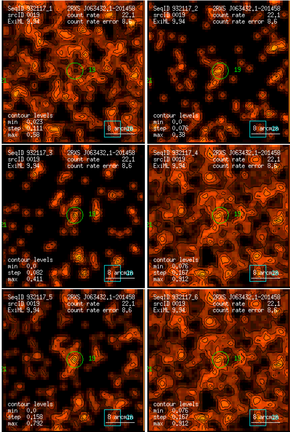
Figure 19: RASS 932117: detection 0019: band rate images, Gaussian filter: (1) PSPC channels 11 – 41, (2) 52 – 90, (3) 91 – 201, (4) 11 – 235, (5) 52 – 201, (6) 11 – 201. Broad band rates in counts/ks. Band rate contour levels in counts/ks/arcmin 2 .
