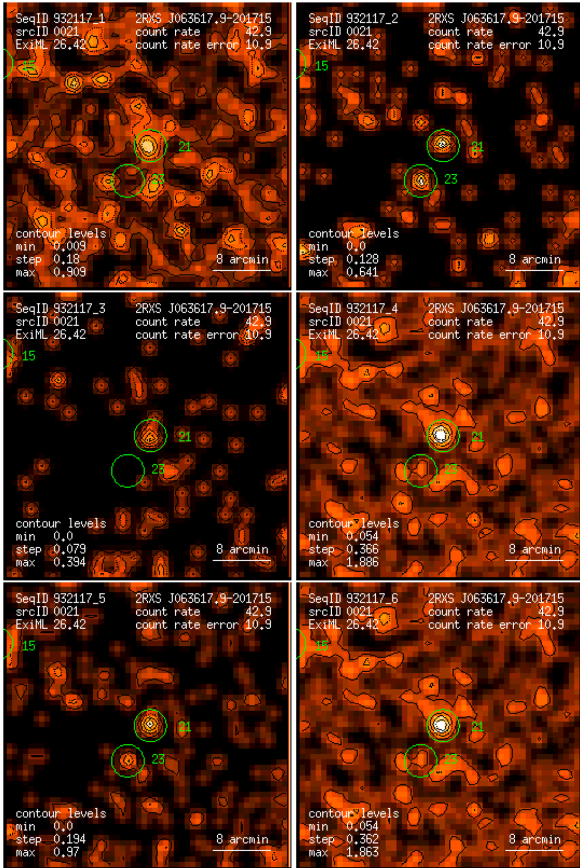
Figure 21: RASS 932117: detection 0021: band rate images, Gaussian filter: (1) PSPC channels 11 – 41, (2) 52 – 90, (3) 91 – 201, (4) 11 – 235, (5) 52 – 201, (6) 11 – 201. Broad band rates in counts/ks. Band rate contour levels in counts/ks/arcmin 2 .
