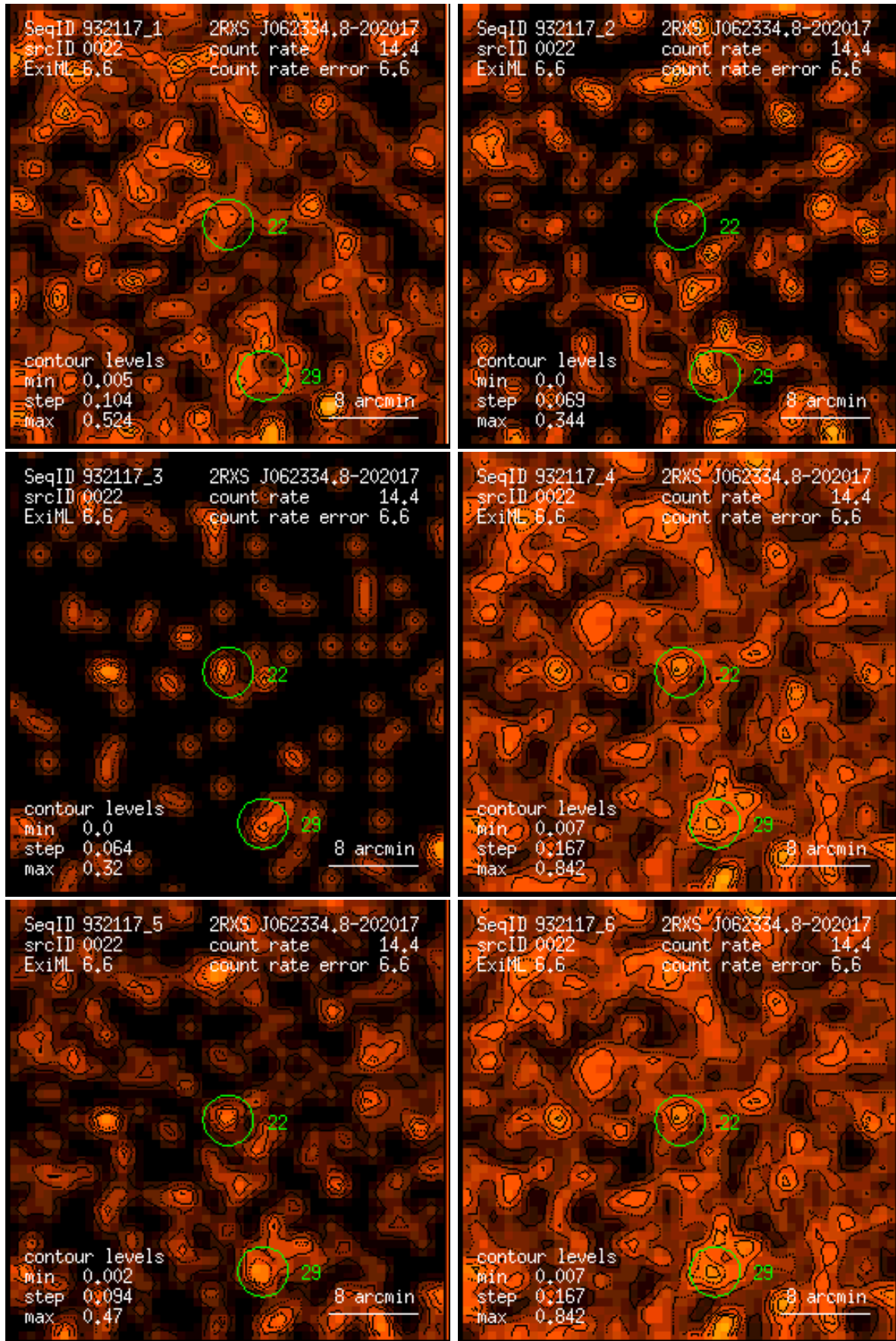
Figure 22: RASS 932117: detection 0022: band rate images, Gaussian filter: (1) PSPC channels 11 – 41, (2) 52 – 90, (3) 91 – 201, (4) 11 – 235, (5) 52 – 201, (6) 11 – 201. Broad band rates in counts/ks. Band rate contour levels in counts/ks/arcmin 2 .
