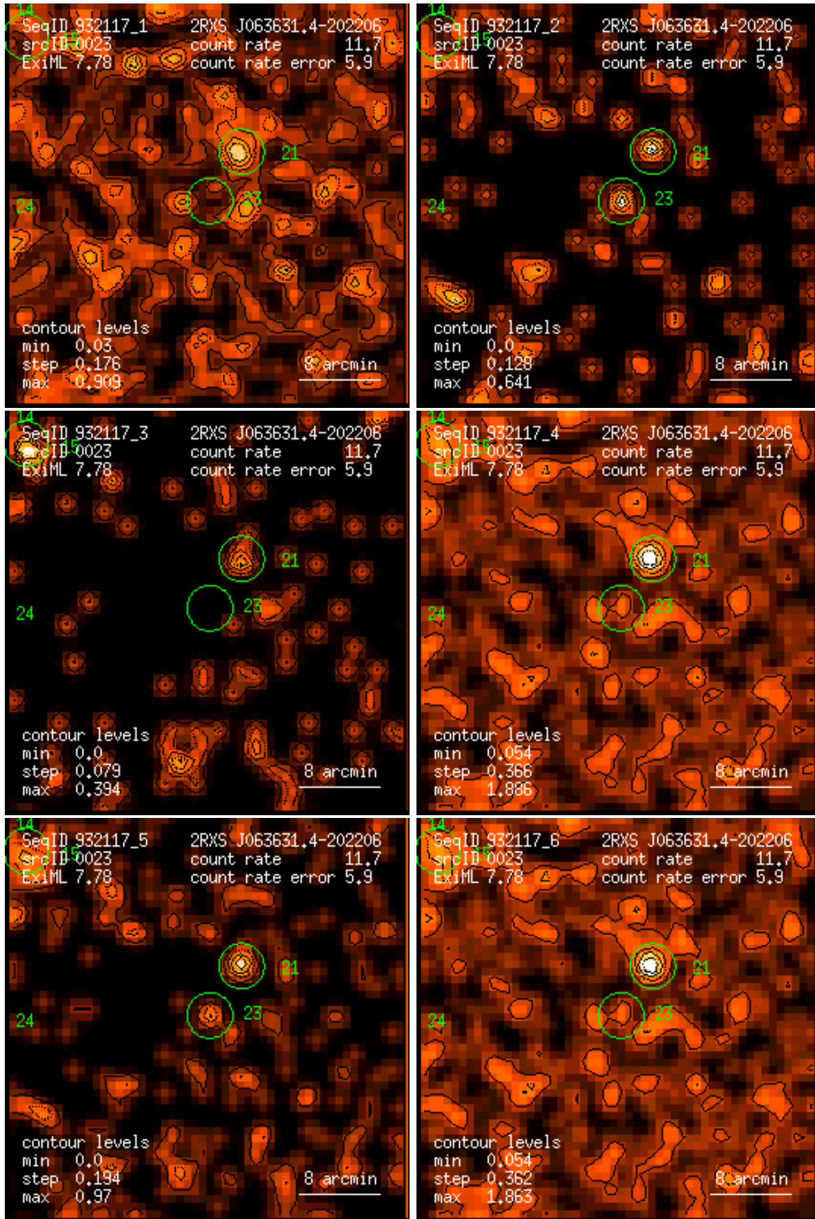
Figure 23: RASS 932117: detection 0023: band rate images, Gaussian filter: (1) PSPC channels 11 – 41, (2) 52 – 90, (3) 91 – 201, (4) 11 – 235, (5) 52 – 201, (6) 11 – 201. Broad band rates in counts/ks. Band rate contour levels in counts/ks/arcmin 2 .
