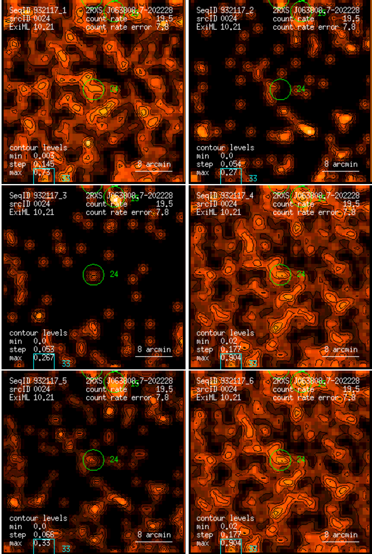
Figure 24: RASS 932117: detection 0024: band rate images, Gaussian filter: (1) PSPC channels 11 – 41, (2) 52 – 90, (3) 91 – 201, (4) 11 – 235, (5) 52 – 201, (6) 11 – 201. Broad band rates in counts/ks. Band rate contour levels in counts/ks/arcmin 2 .
