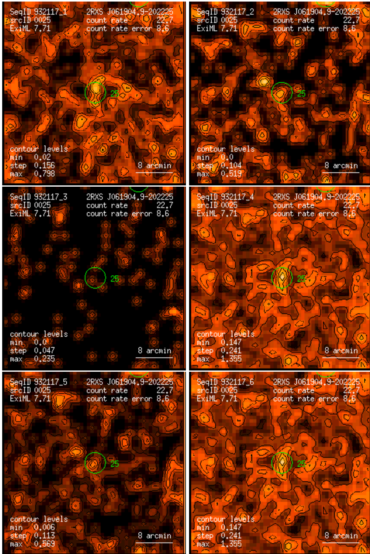
Figure 25: RASS 932117: detection 0025: band rate images, Gaussian filter: (1) PSPC channels 11 – 41, (2) 52 – 90, (3) 91 – 201, (4) 11 – 235, (5) 52 – 201, (6) 11 – 201. Broad band rates in counts/ks. Band rate contour levels in counts/ks/arcmin 2 .
