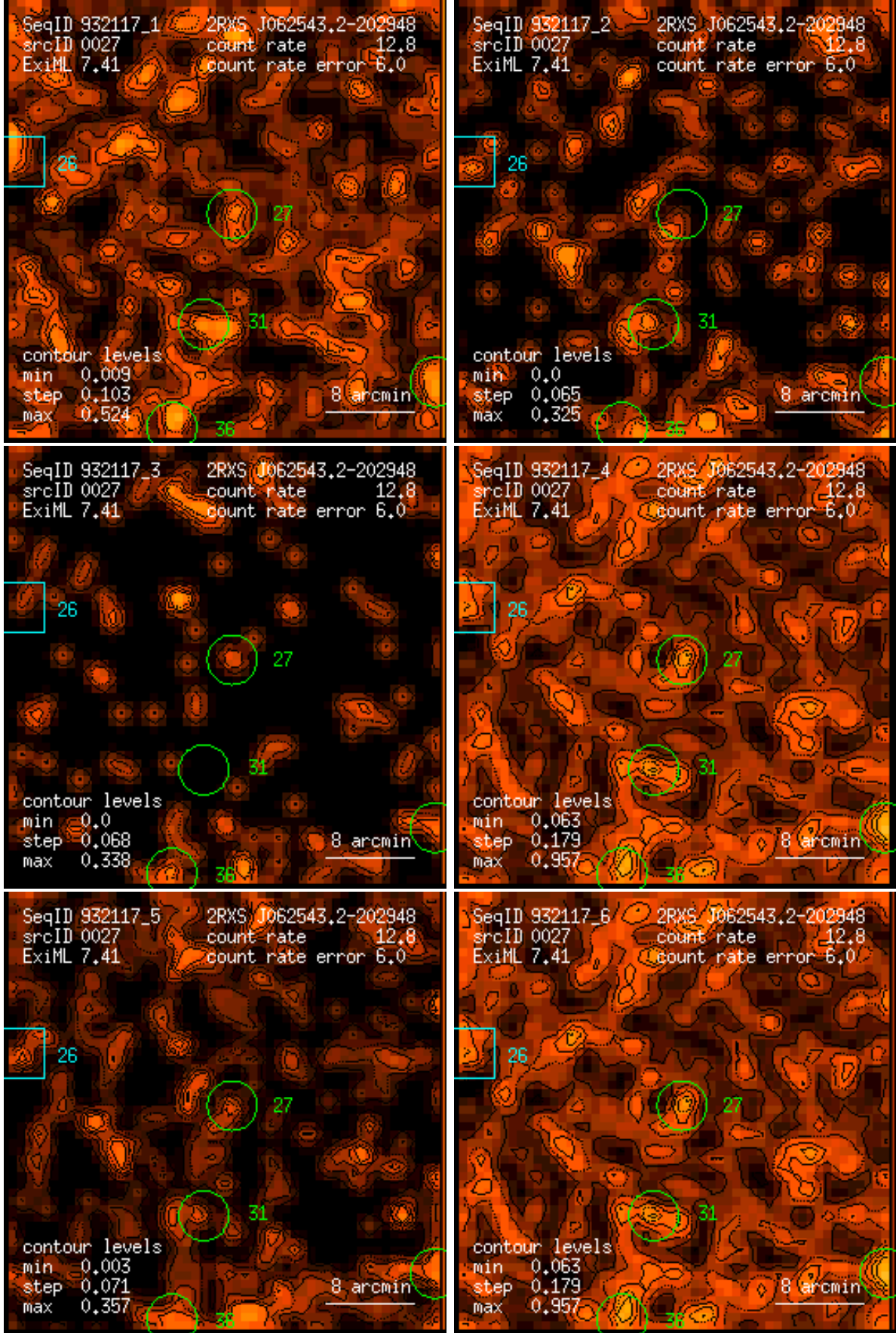
Figure 27: RASS 932117: detection 0027: band rate images, Gaussian filter: (1) PSPC channels 11 – 41, (2) 52 – 90, (3) 91 – 201, (4) 11 – 235, (5) 52 – 201, (6) 11 – 201. Broad band rates in counts/ks. Band rate contour levels in counts/ks/arcmin 2 .
