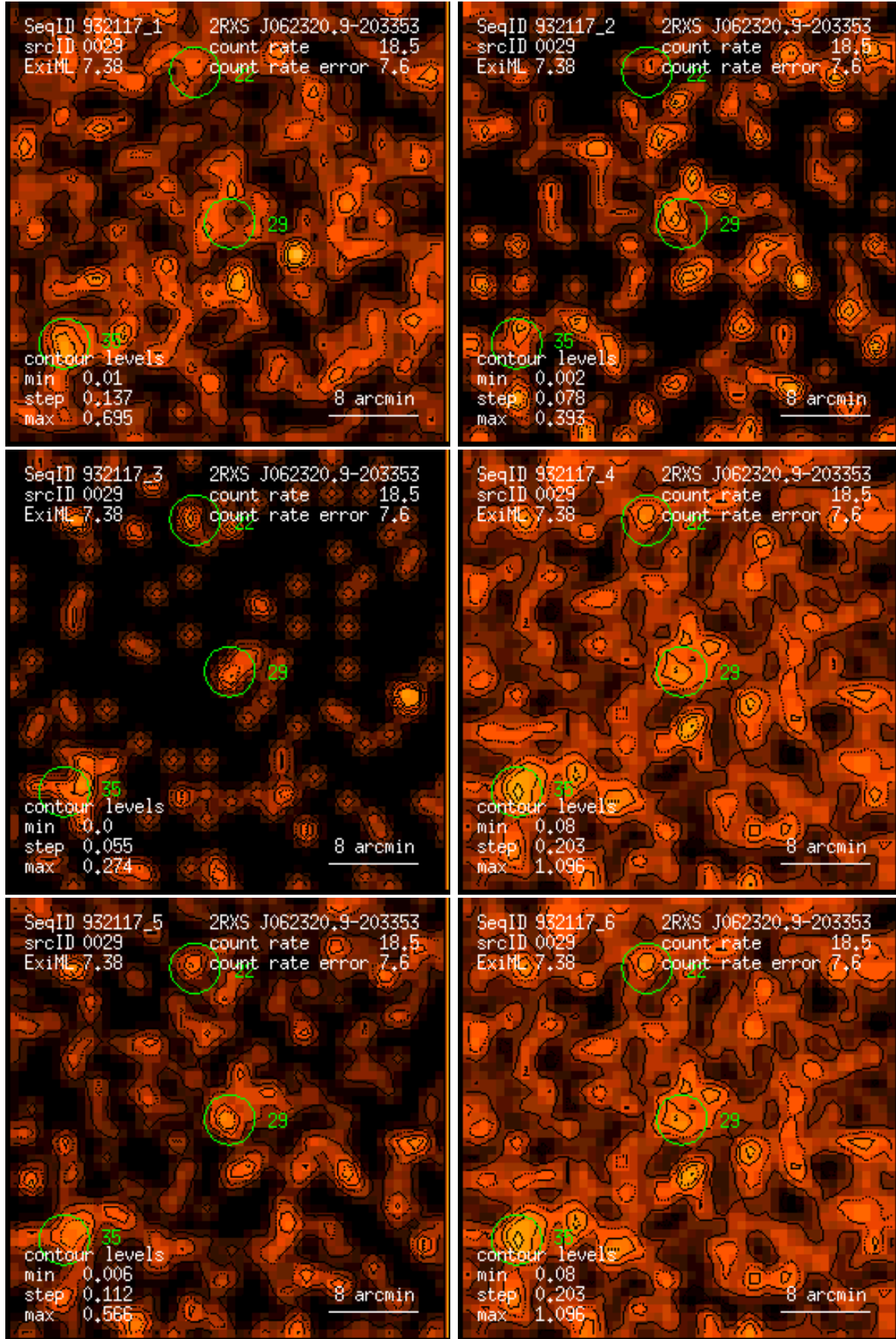
Figure 29: RASS 932117: detection 0029: band rate images, Gaussian filter: (1) PSPC channels 11 – 41, (2) 52 – 90, (3) 91 – 201, (4) 11 – 235, (5) 52 – 201, (6) 11 – 201. Broad band rates in counts/ks. Band rate contour levels in counts/ks/arcmin 2 .
