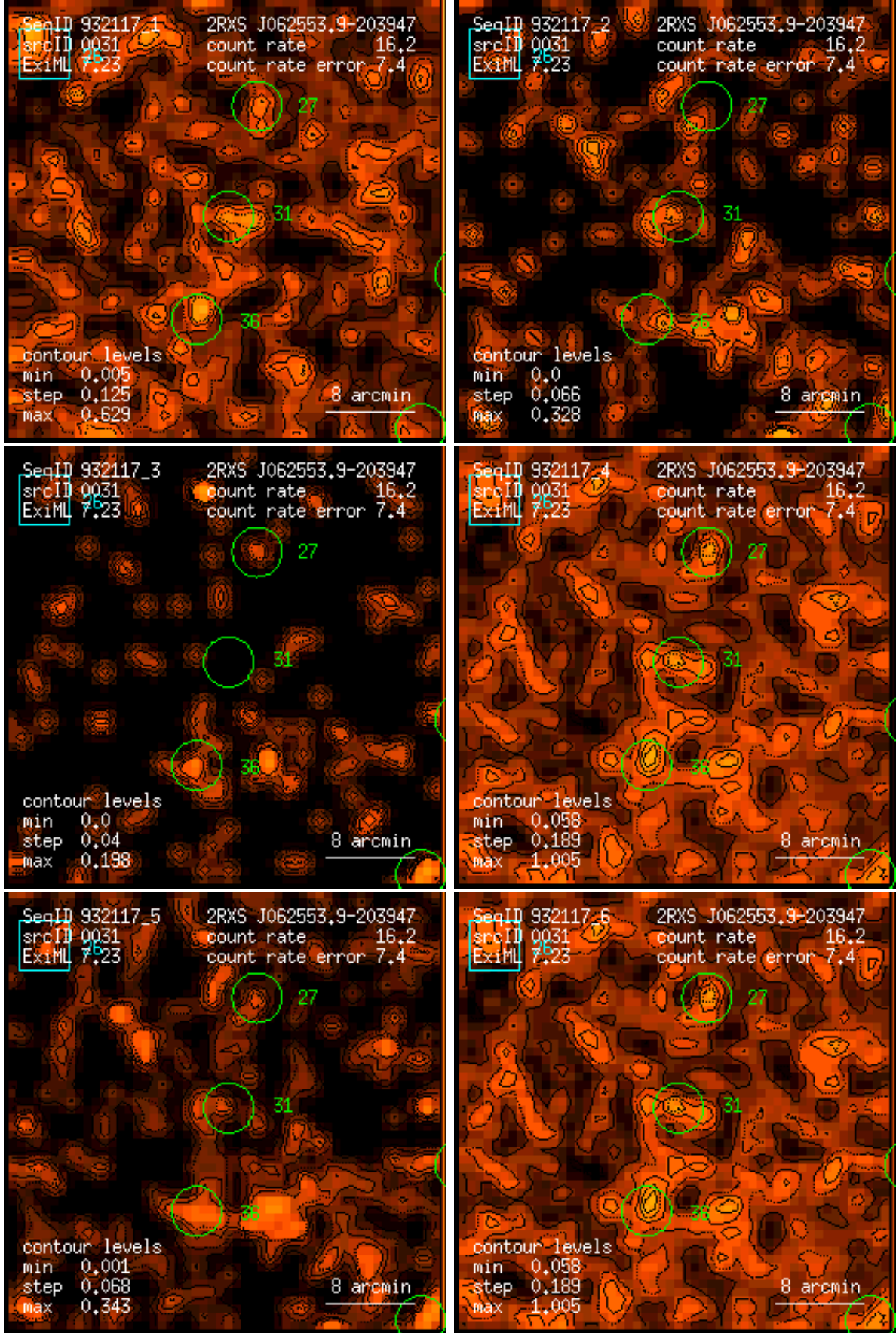
Figure 31: RASS 932117: detection 0031: band rate images, Gaussian filter: (1) PSPC channels 11 – 41, (2) 52 – 90, (3) 91 – 201, (4) 11 – 235, (5) 52 – 201, (6) 11 – 201. Broad band rates in counts/ks. Band rate contour levels in counts/ks/arcmin 2 .
