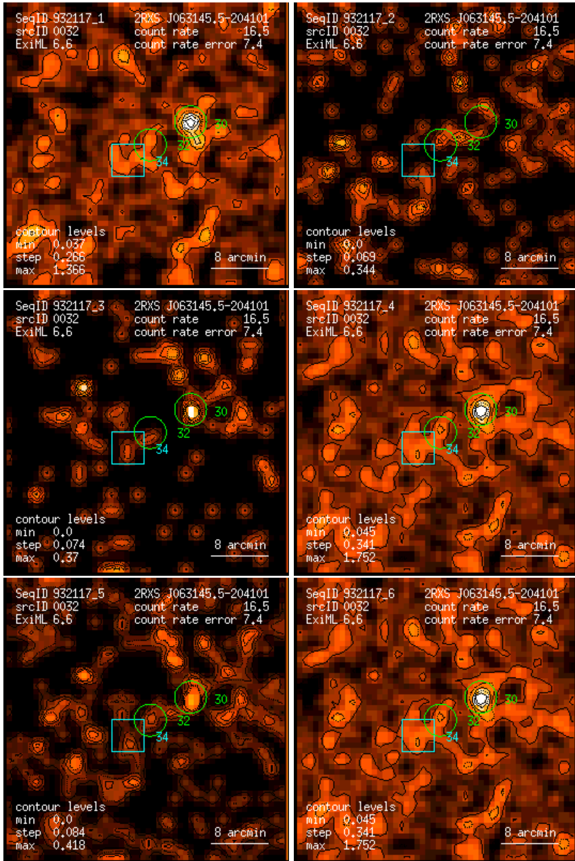
Figure 32: RASS 932117: detection 0032: band rate images, Gaussian filter: (1) PSPC channels 11 – 41, (2) 52 – 90, (3) 91 – 201, (4) 11 – 235, (5) 52 – 201, (6) 11 – 201. Broad band rates in counts/ks. Band rate contour levels in counts/ks/arcmin 2 .
