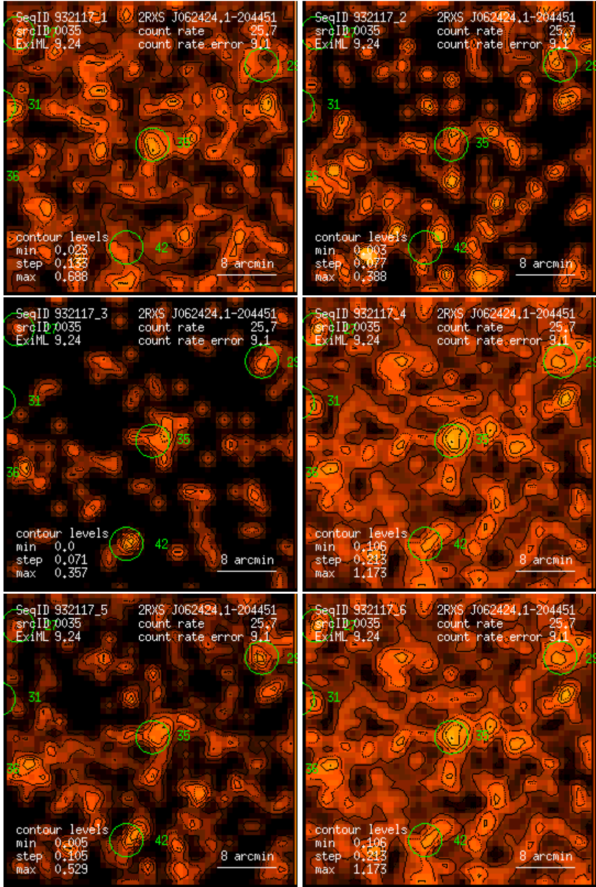
Figure 35: RASS 932117: detection 0035: band rate images, Gaussian filter: (1) PSPC channels 11 – 41, (2) 52 – 90, (3) 91 – 201, (4) 11 – 235, (5) 52 – 201, (6) 11 – 201. Broad band rates in counts/ks. Band rate contour levels in counts/ks/arcmin 2 .
