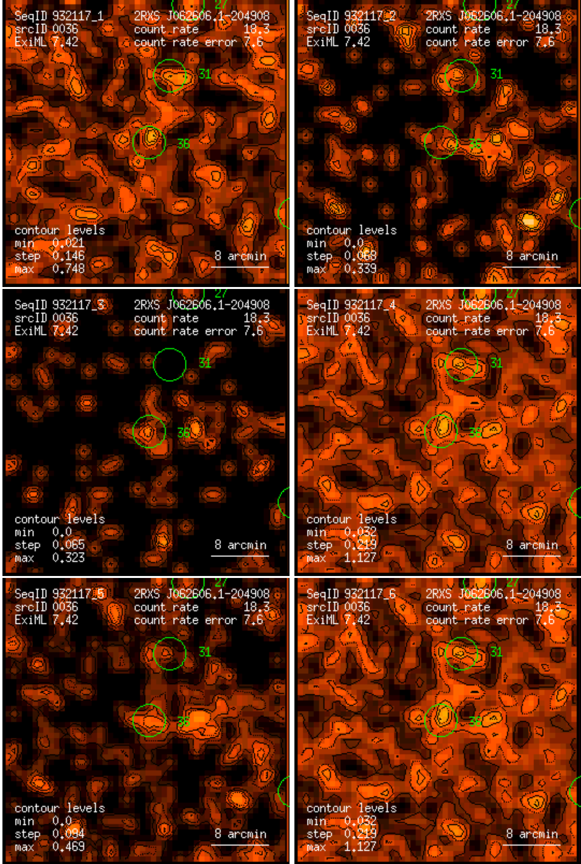
Figure 36: RASS 932117: detection 0036: band rate images, Gaussian filter: (1) PSPC channels 11 – 41, (2) 52 – 90, (3) 91 – 201, (4) 11 – 235, (5) 52 – 201, (6) 11 – 201. Broad band rates in counts/ks. Band rate contour levels in counts/ks/arcmin 2 .
