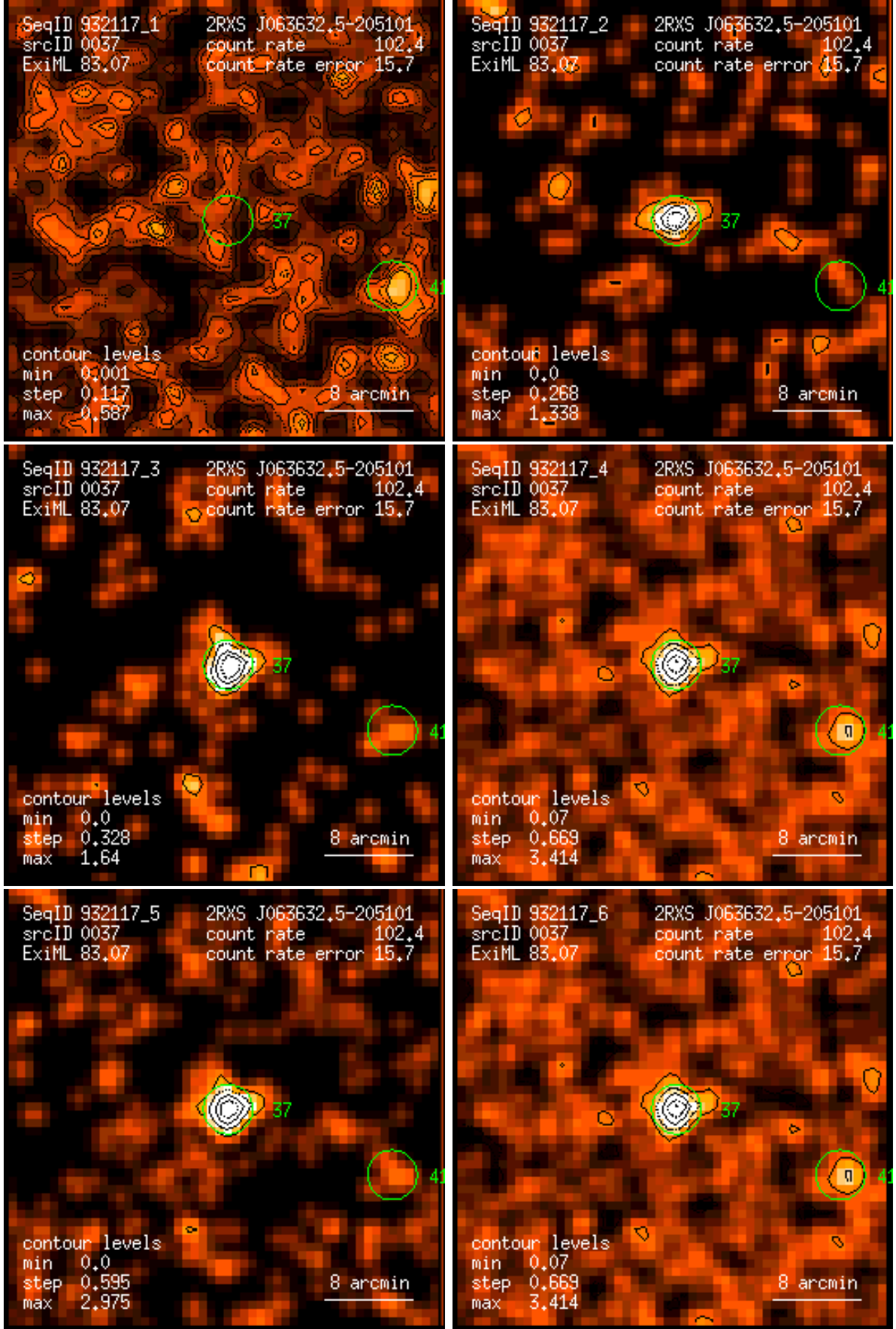
Figure 37: RASS 932117: detection 0037: band rate images, Gaussian filter: (1) PSPC channels 11 – 41, (2) 52 – 90, (3) 91 – 201, (4) 11 – 235, (5) 52 – 201, (6) 11 – 201. Broad band rates in counts/ks. Band rate contour levels in counts/ks/arcmin 2 .
