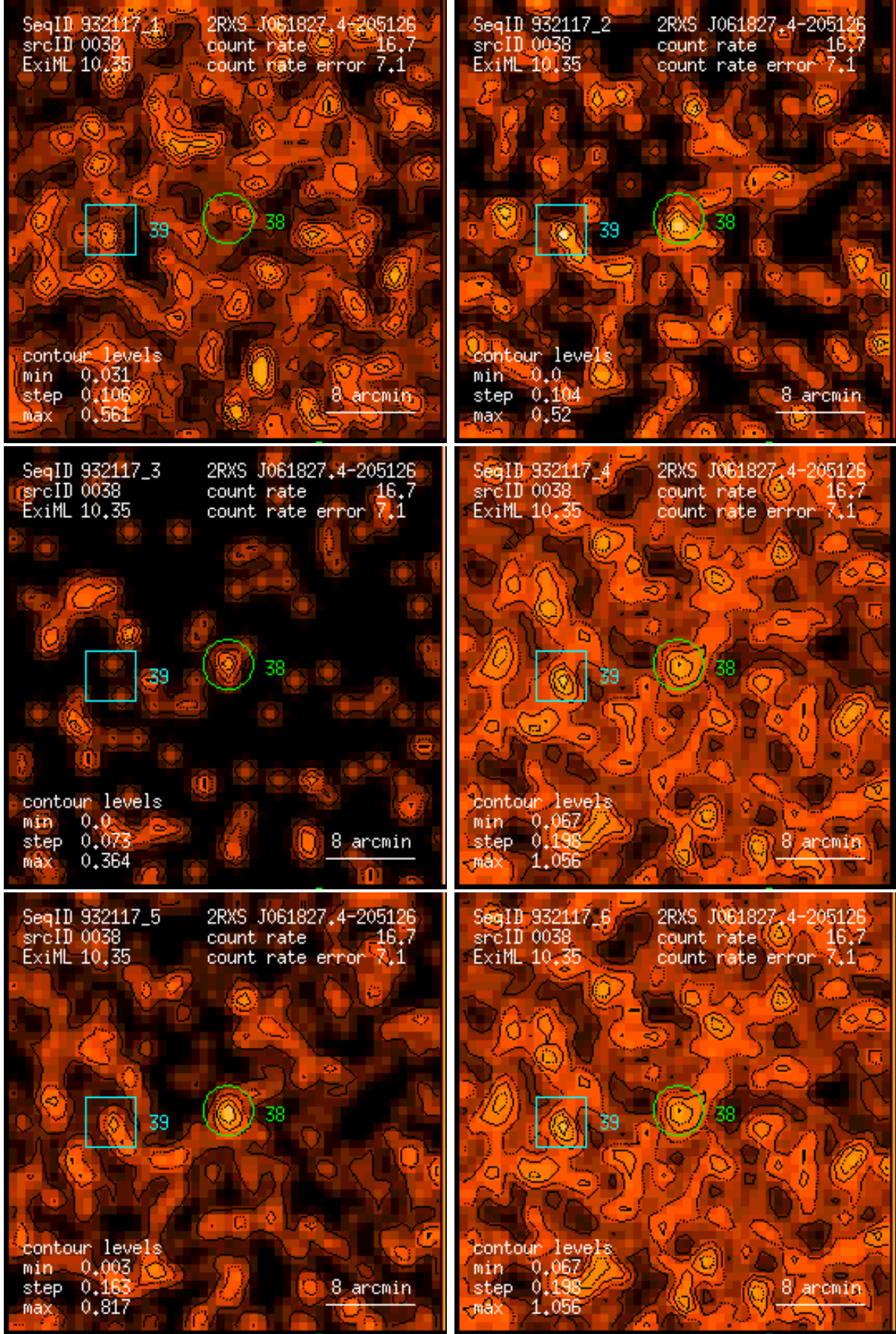
Figure 38: RASS 932117: detection 0038: band rate images, Gaussian filter: (1) PSPC channels 11 – 41, (2) 52 – 90, (3) 91 – 201, (4) 11 – 235, (5) 52 – 201, (6) 11 – 201. Broad band rates in counts/ks. Band rate contour levels in counts/ks/arcmin 2 .
