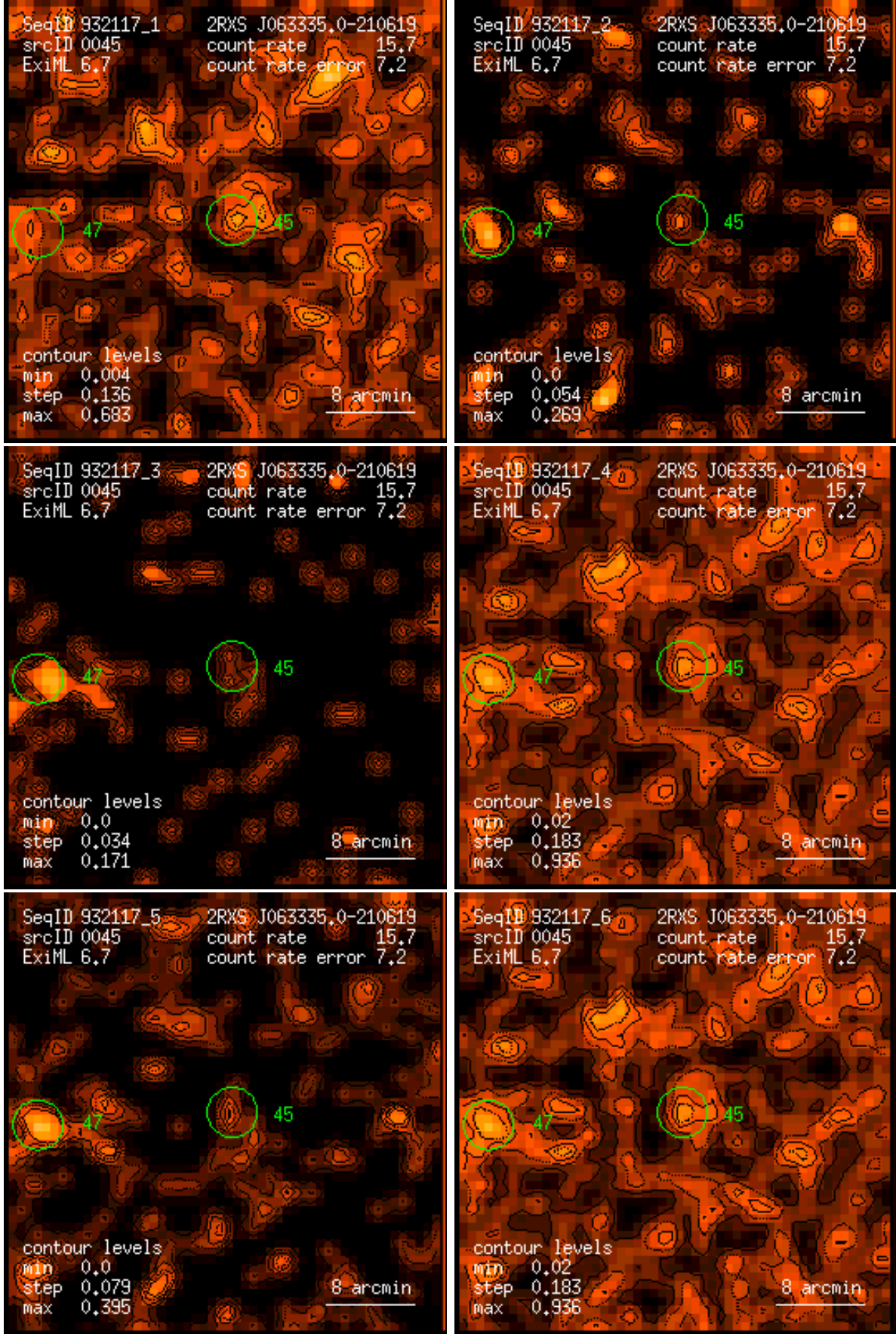
Figure 45: RASS 932117: detection 0045: band rate images, Gaussian filter: (1) PSPC channels 11 – 41, (2) 52 – 90, (3) 91 – 201, (4) 11 – 235, (5) 52 – 201, (6) 11 – 201. Broad band rates in counts/ks. Band rate contour levels in counts/ks/arcmin 2 .
