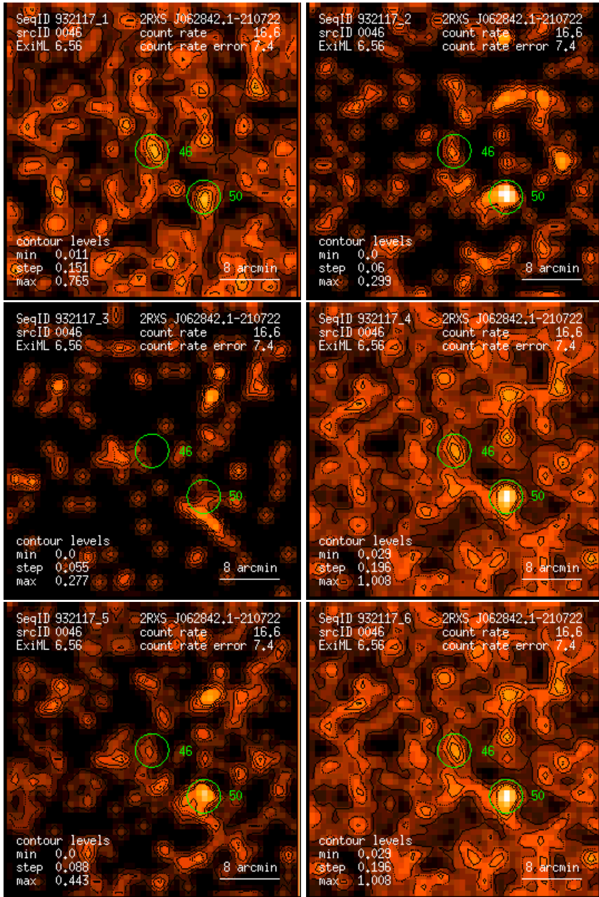
Figure 46: RASS 932117: detection 0046: band rate images, Gaussian filter: (1) PSPC channels 11 – 41, (2) 52 – 90, (3) 91 – 201, (4) 11 – 235, (5) 52 – 201, (6) 11 – 201. Broad band rates in counts/ks. Band rate contour levels in counts/ks/arcmin 2 .
