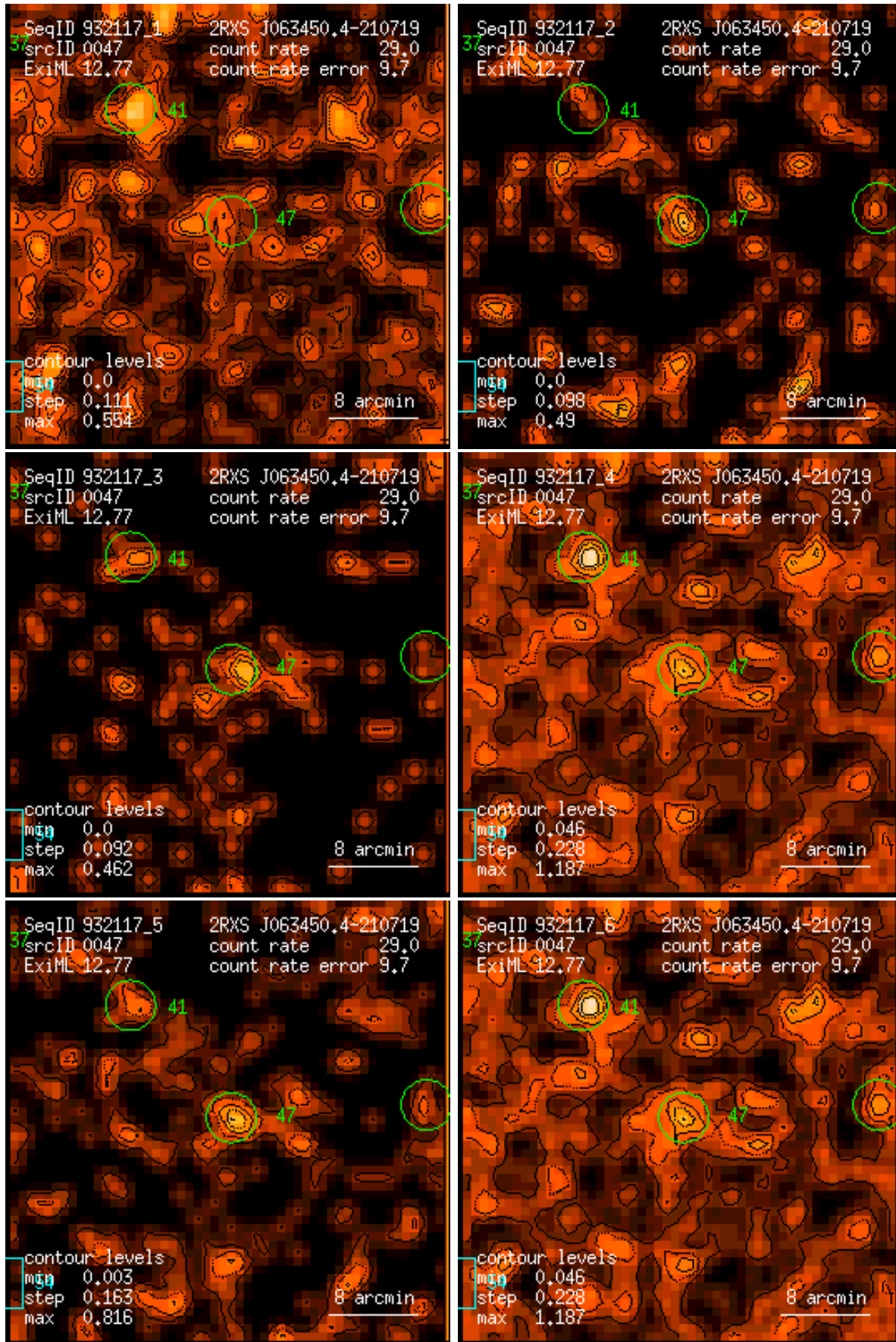
Figure 47: RASS 932117: detection 0047: band rate images, Gaussian filter: (1) PSPC channels 11 – 41, (2) 52 – 90, (3) 91 – 201, (4) 11 – 235, (5) 52 – 201, (6) 11 – 201. Broad band rates in counts/ks. Band rate contour levels in counts/ks/arcmin 2 .
