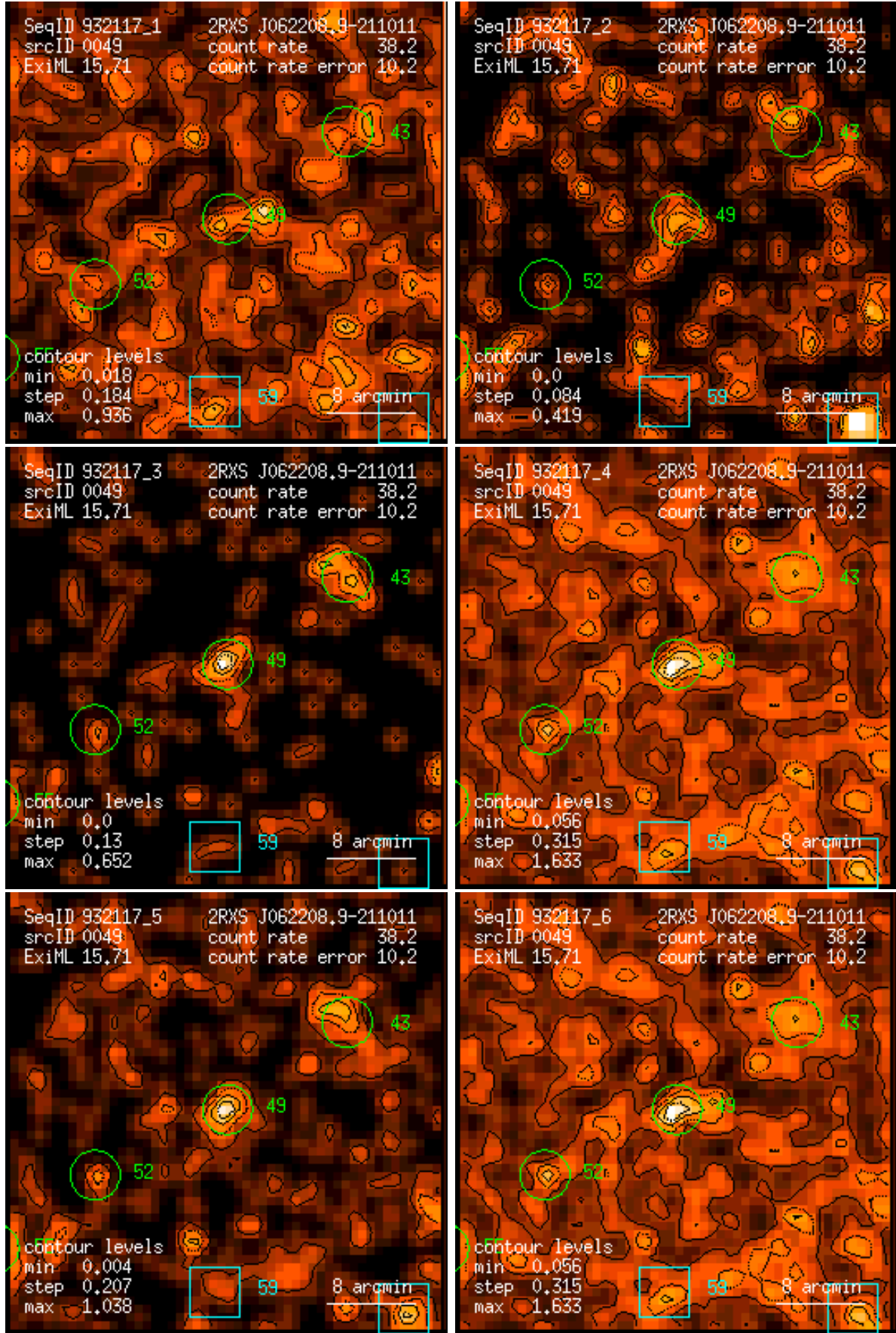
Figure 49: RASS 932117: detection 0049: band rate images, Gaussian filter: (1) PSPC channels 11 – 41, (2) 52 – 90, (3) 91 – 201, (4) 11 – 235, (5) 52 – 201, (6) 11 – 201. Broad band rates in counts/ks. Band rate contour levels in counts/ks/arcmin 2 .
