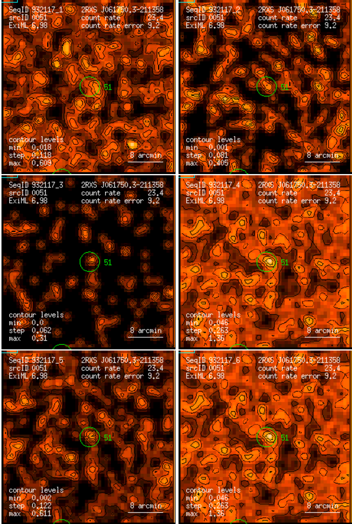
Figure 51: RASS 932117: detection 0051: band rate images, Gaussian filter: (1) PSPC channels 11 – 41, (2) 52 – 90, (3) 91 – 201, (4) 11 – 235, (5) 52 – 201, (6) 11 – 201. Broad band rates in counts/ks. Band rate contour levels in counts/ks/arcmin 2 .
