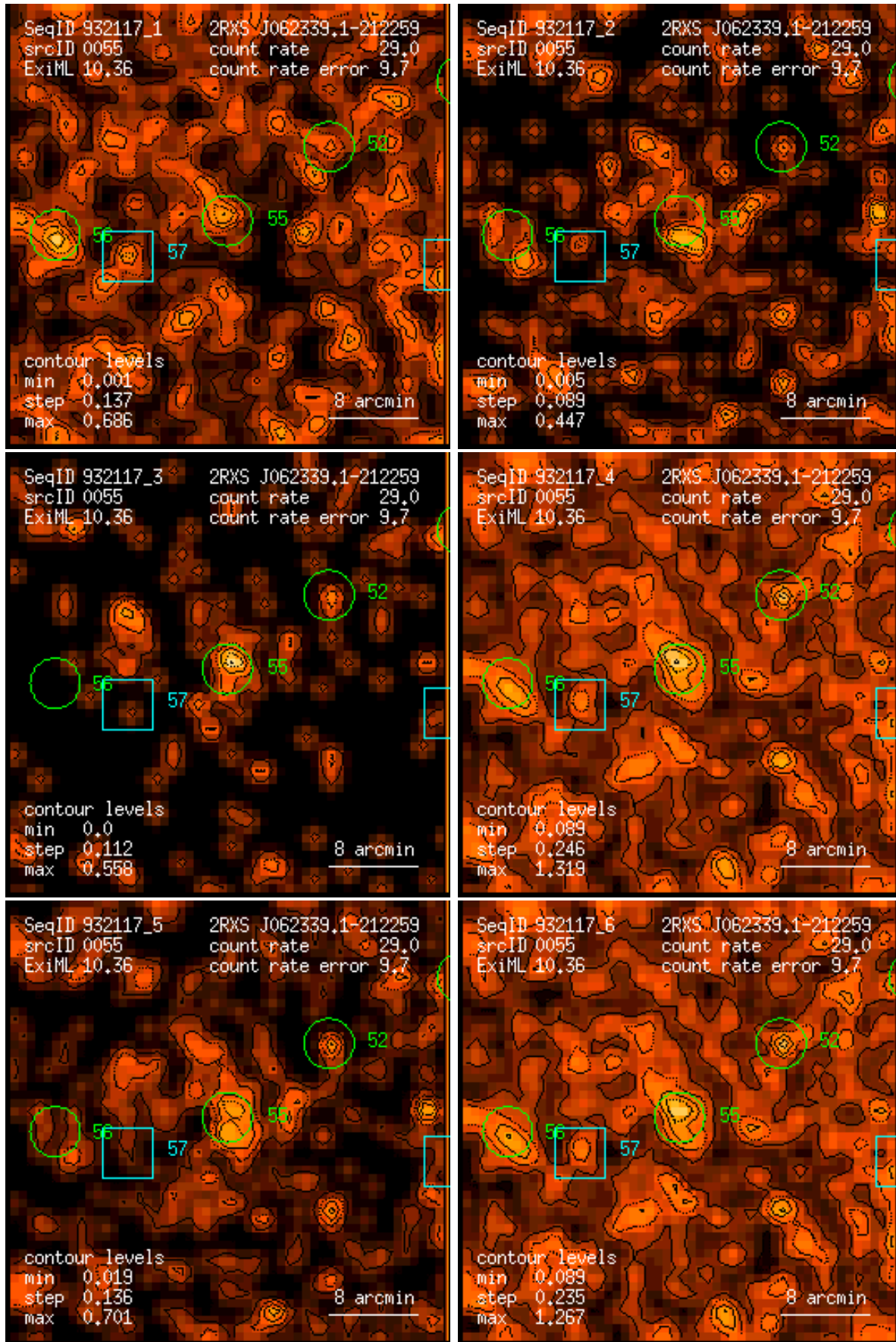
Figure 55: RASS 932117: detection 0055: band rate images, Gaussian filter: (1) PSPC channels 11 – 41, (2) 52 – 90, (3) 91 – 201, (4) 11 – 235, (5) 52 – 201, (6) 11 – 201. Broad band rates in counts/ks. Band rate contour levels in counts/ks/arcmin 2 .
