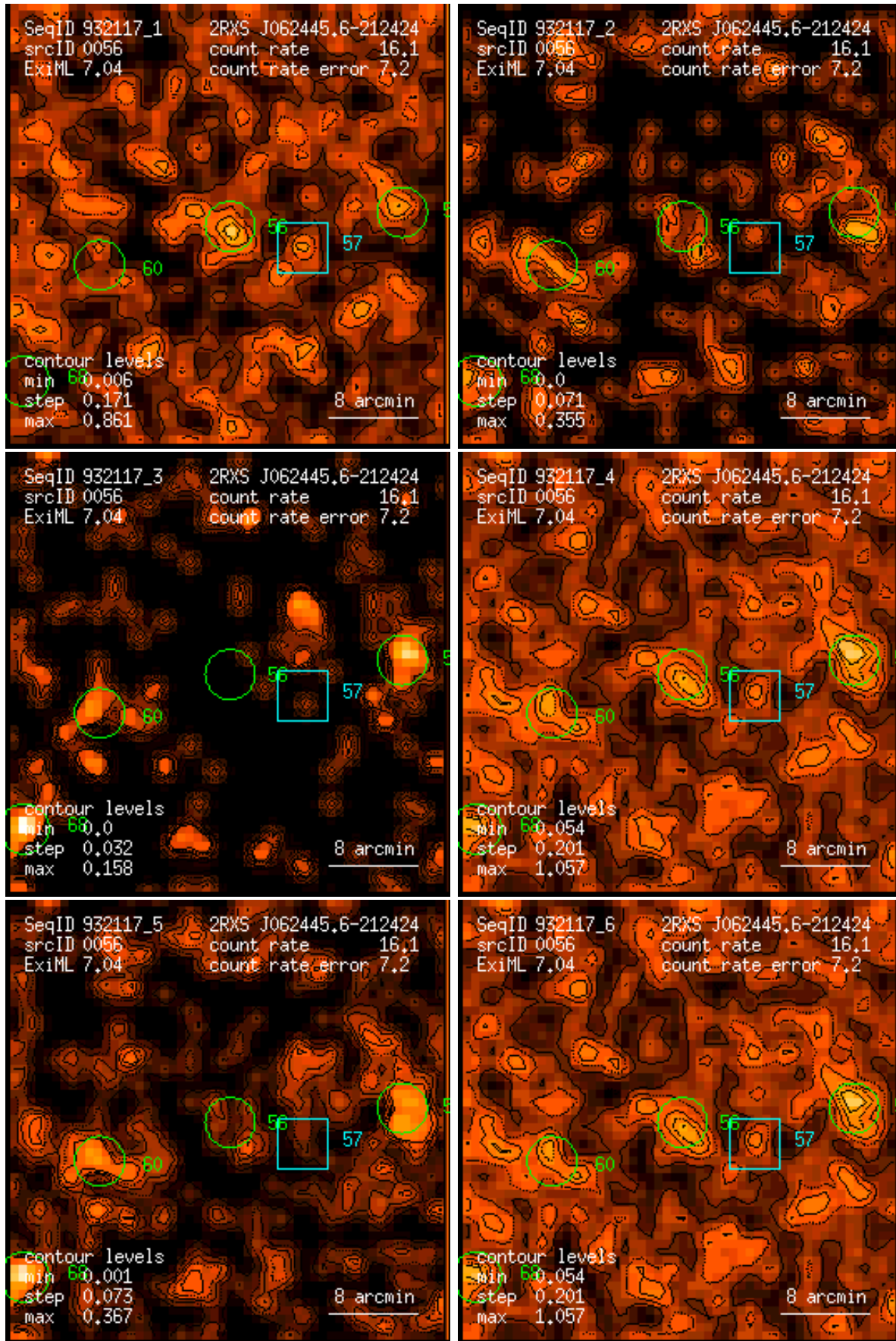
Figure 56: RASS 932117: detection 0056: band rate images, Gaussian filter: (1) PSPC channels 11 – 41, (2) 52 – 90, (3) 91 – 201, (4) 11 – 235, (5) 52 – 201, (6) 11 – 201. Broad band rates in counts/ks. Band rate contour levels in counts/ks/arcmin 2 .
