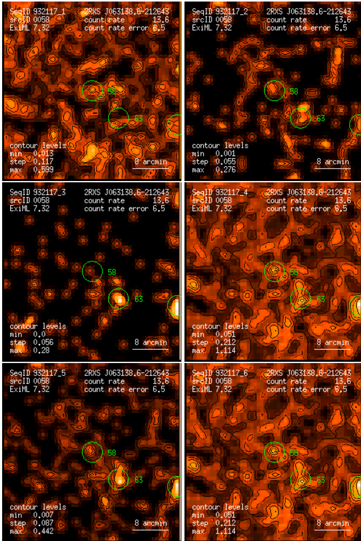
Figure 58: RASS 932117: detection 0058: band rate images, Gaussian filter: (1) PSPC channels 11 – 41, (2) 52 – 90, (3) 91 – 201, (4) 11 – 235, (5) 52 – 201, (6) 11 – 201. Broad band rates in counts/ks. Band rate contour levels in counts/ks/arcmin 2 .
