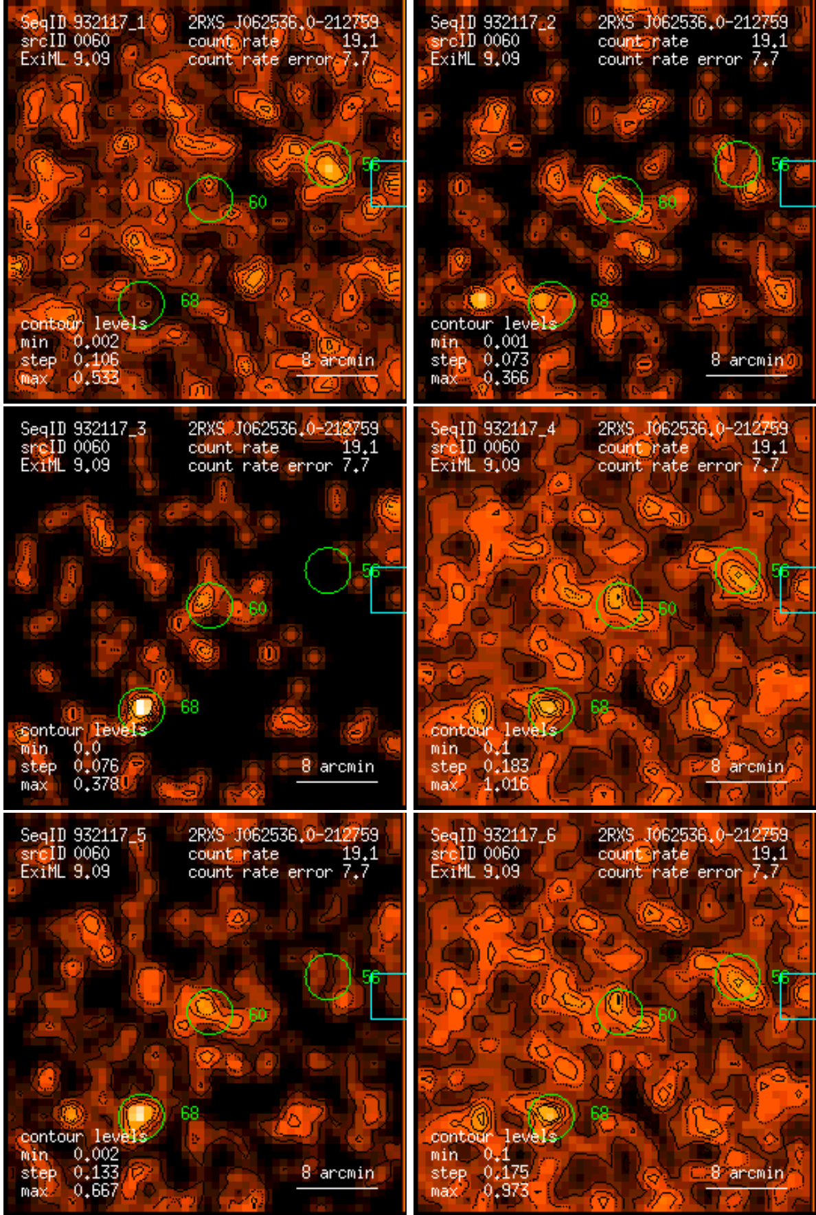
Figure 60: RASS 932117: detection 0060: band rate images, Gaussian filter: (1) PSPC channels 11 – 41, (2) 52 – 90, (3) 91 – 201, (4) 11 – 235, (5) 52 – 201, (6) 11 – 201. Broad band rates in counts/ks. Band rate contour levels in counts/ks/arcmin 2 .
