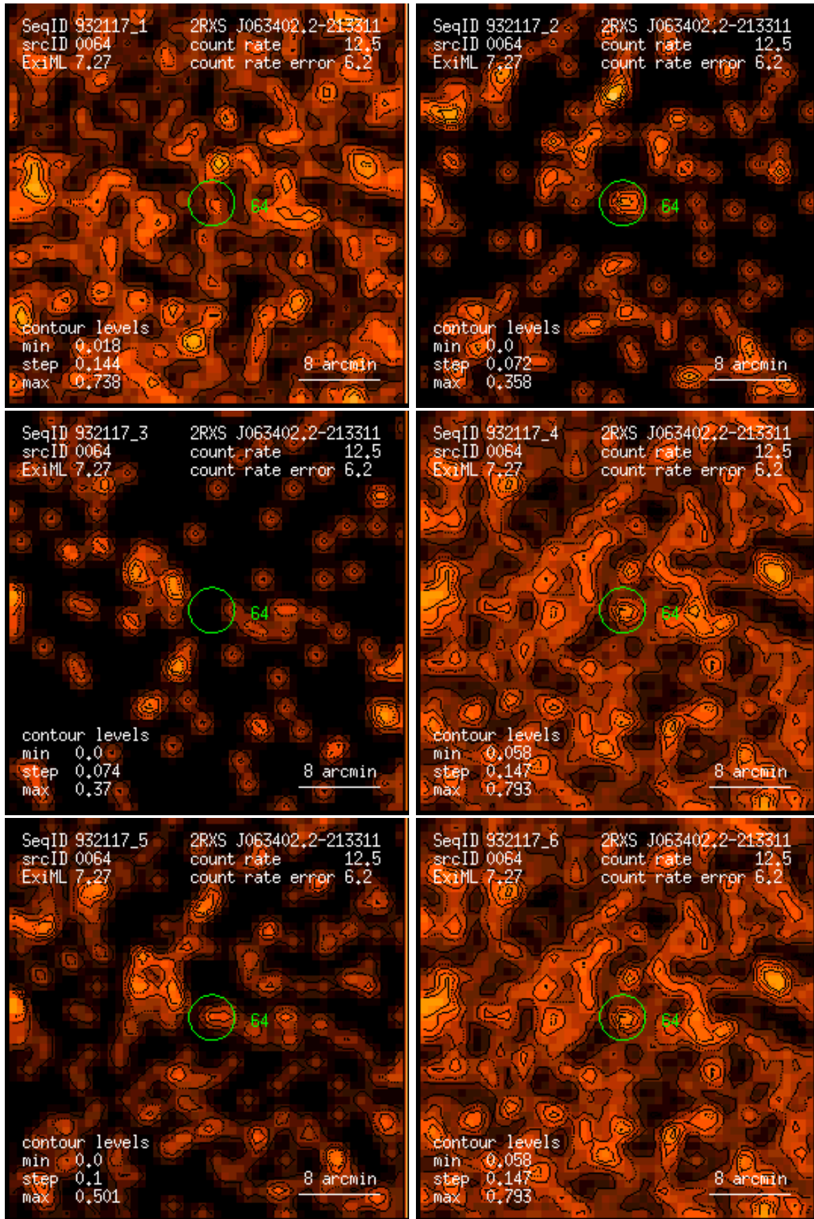
Figure 64: RASS 932117: detection 0064: band rate images, Gaussian filter: (1) PSPC channels 11 – 41, (2) 52 – 90, (3) 91 – 201, (4) 11 – 235, (5) 52 – 201, (6) 11 – 201. Broad band rates in counts/ks. Band rate contour levels in counts/ks/arcmin 2 .
