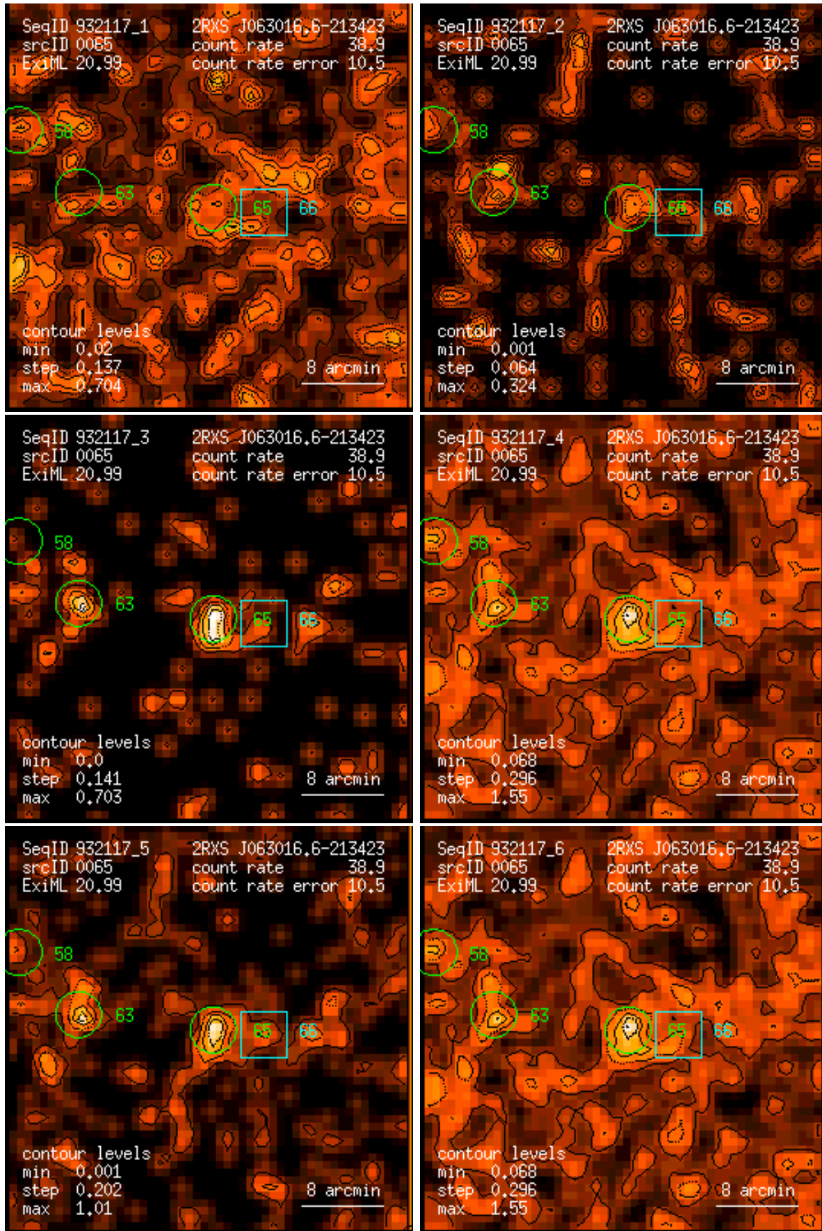
Figure 65: RASS 932117: detection 0065: band rate images, Gaussian filter: (1) PSPC channels 11 – 41, (2) 52 – 90, (3) 91 – 201, (4) 11 – 235, (5) 52 – 201, (6) 11 – 201. Broad band rates in counts/ks. Band rate contour levels in counts/ks/arcmin 2 .
