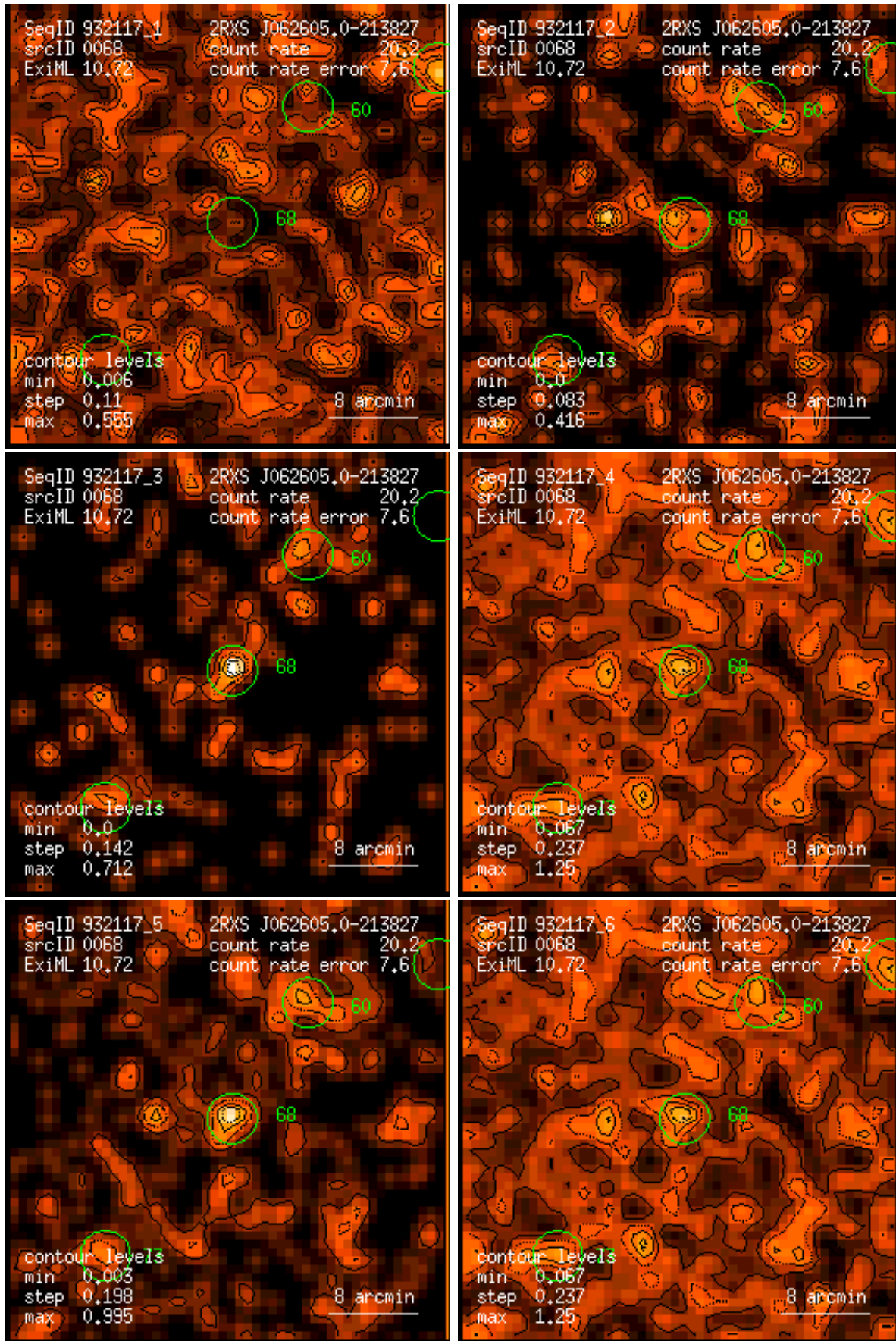
Figure 68: RASS 932117: detection 0068: band rate images, Gaussian filter: (1) PSPC channels 11 – 41, (2) 52 – 90, (3) 91 – 201, (4) 11 – 235, (5) 52 – 201, (6) 11 – 201. Broad band rates in counts/ks. Band rate contour levels in counts/ks/arcmin 2 .
