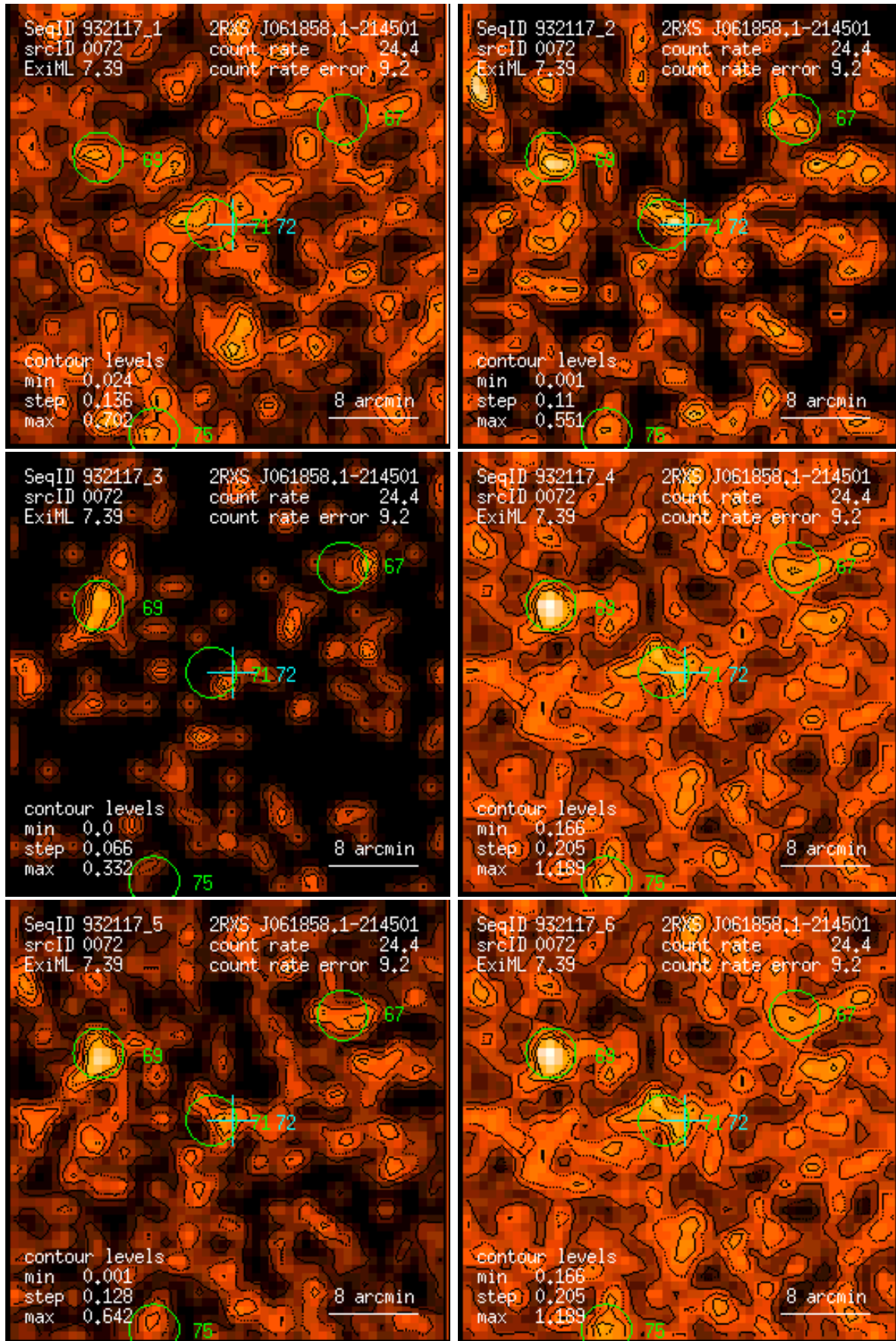
Figure 72: RASS 932117: detection 0072: band rate images, Gaussian filter: (1) PSPC channels 11 – 41, (2) 52 – 90, (3) 91 – 201, (4) 11 – 235, (5) 52 – 201, (6) 11 – 201. Broad band rates in counts/ks. Band rate contour levels in counts/ks/arcmin 2 .
