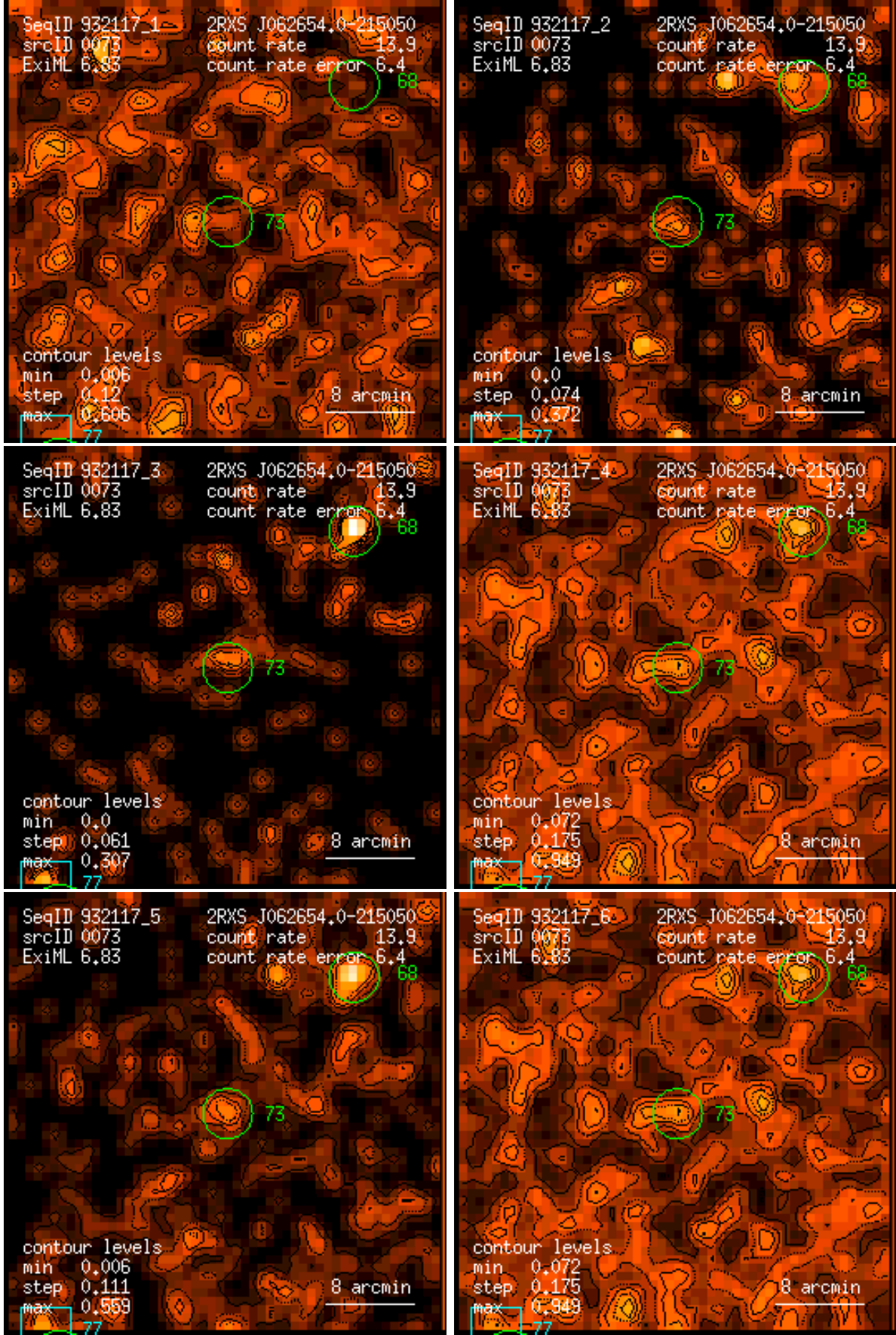
Figure 73: RASS 932117: detection 0073: band rate images, Gaussian filter: (1) PSPC channels 11 – 41, (2) 52 – 90, (3) 91 – 201, (4) 11 – 235, (5) 52 – 201, (6) 11 – 201. Broad band rates in counts/ks. Band rate contour levels in counts/ks/arcmin 2 .
